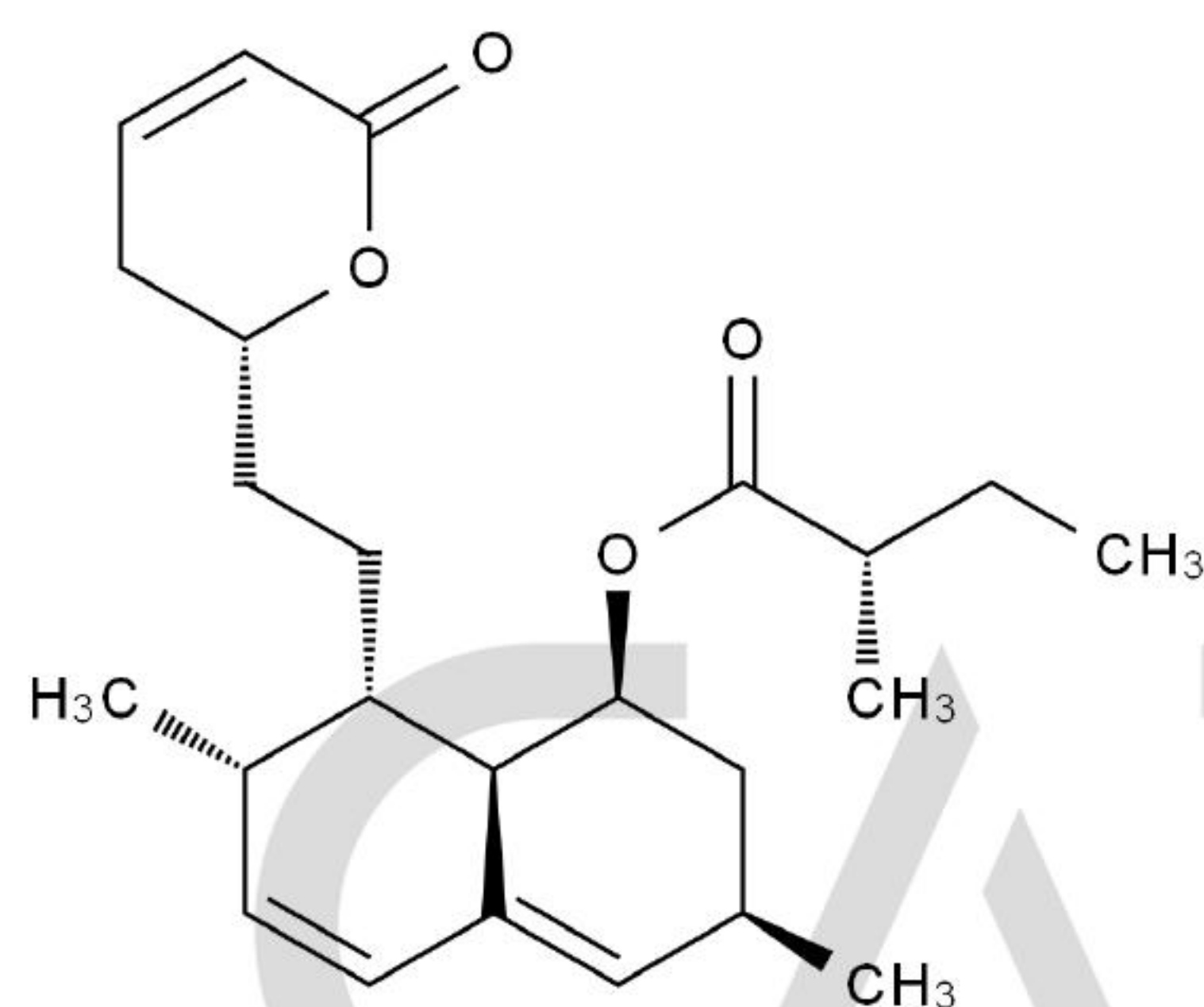
Chemical Structure:
