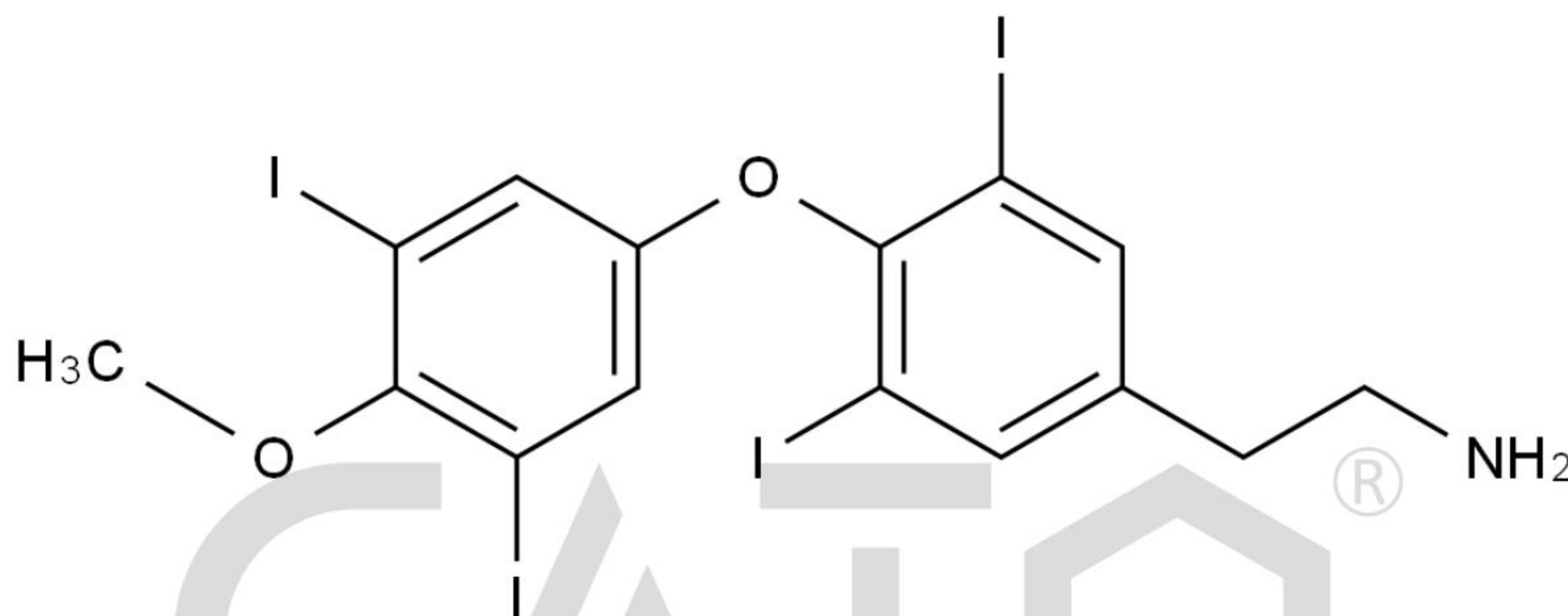
Chemical Structure:
