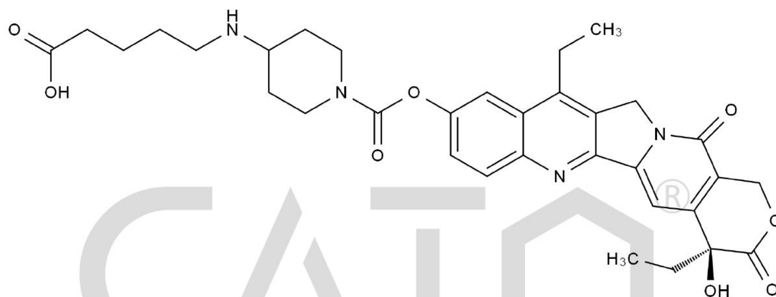
Chemical Structure:
