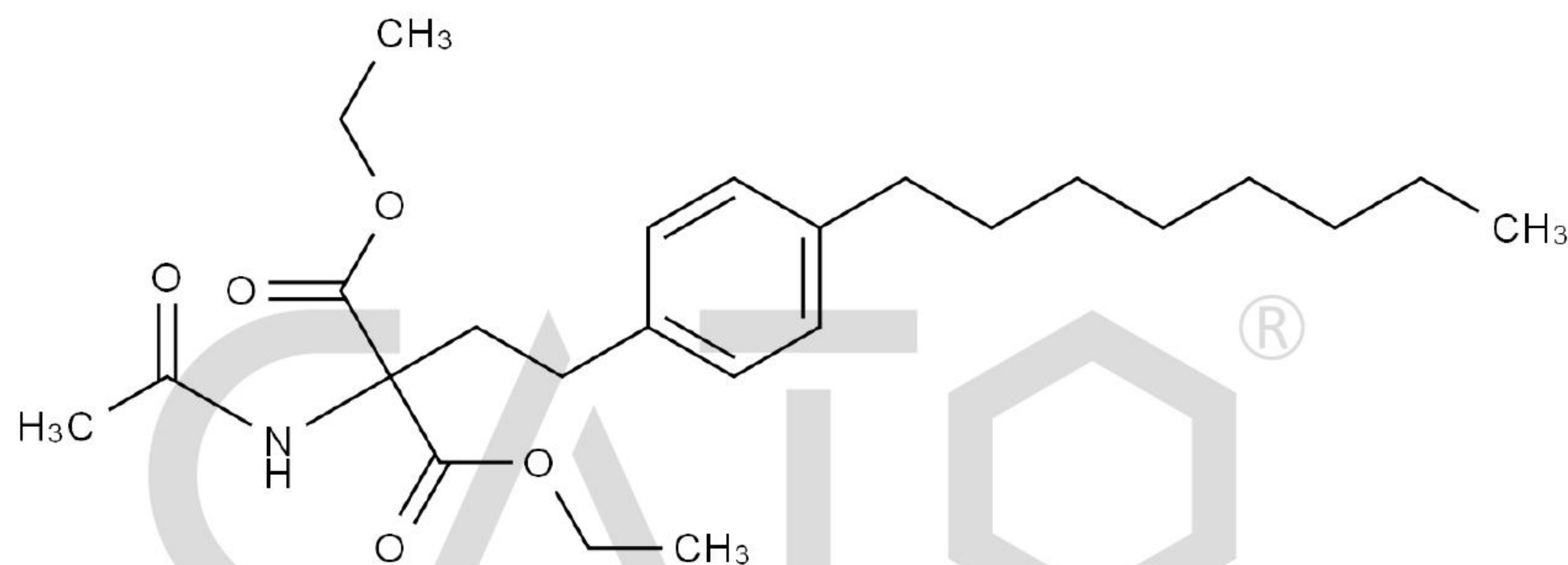
Chemical Structure:
