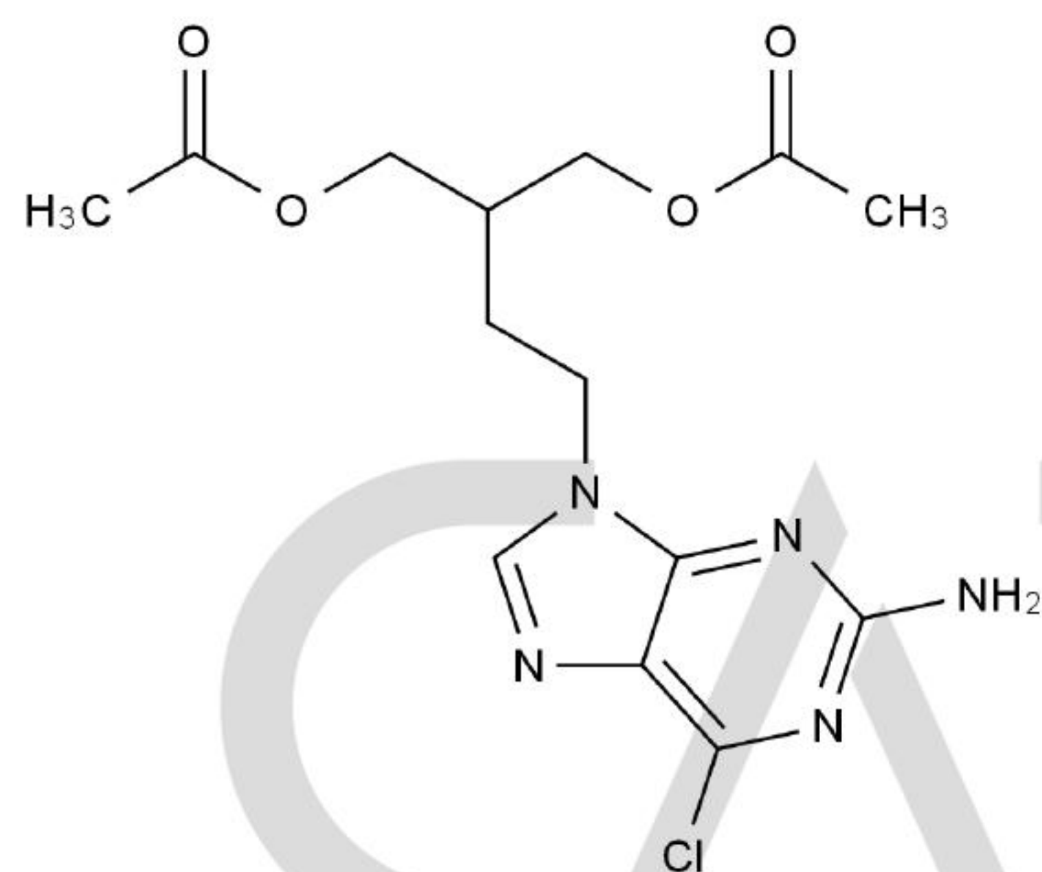
Chemical Structure:
