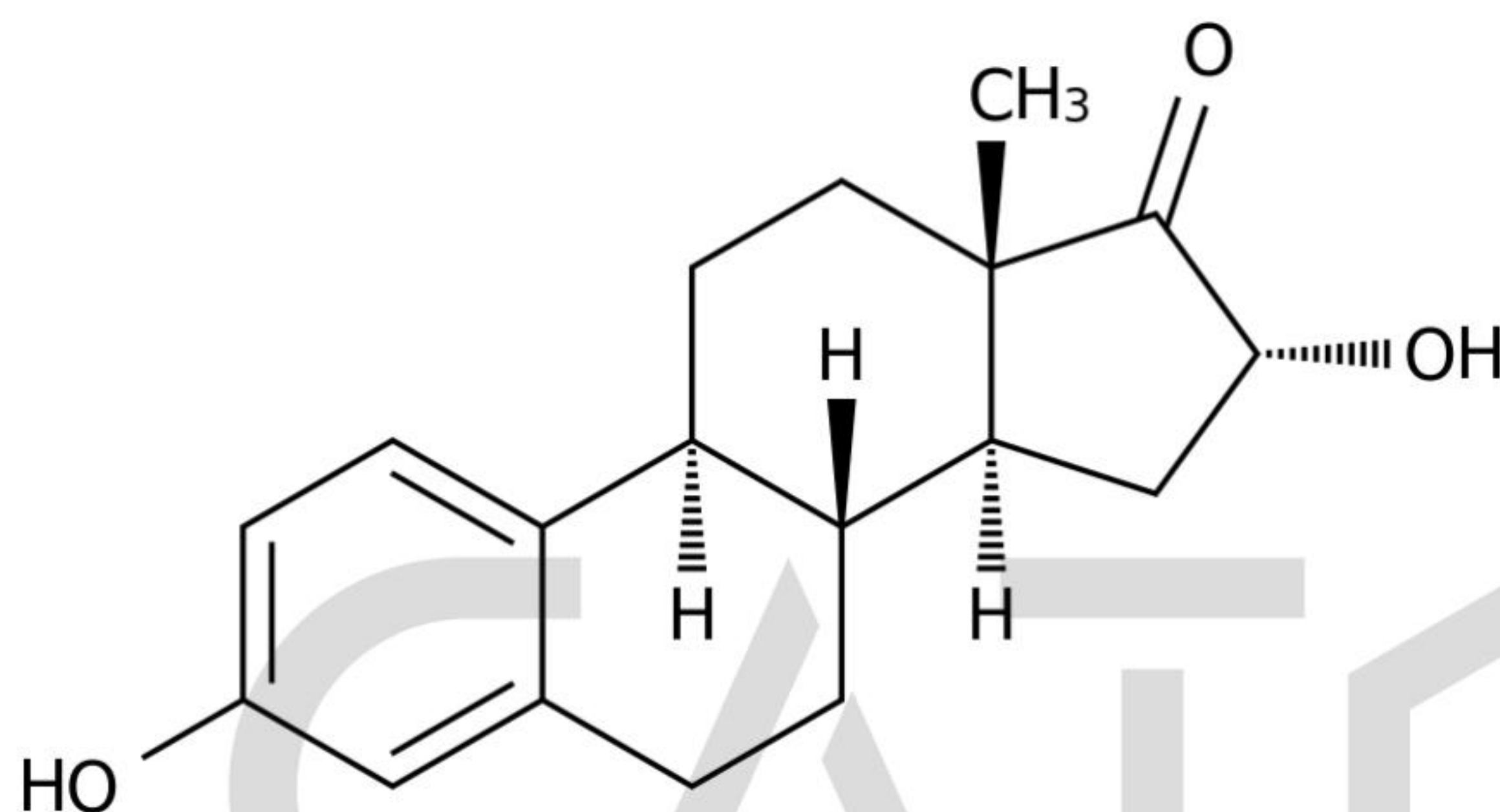
Chemical Structure:
