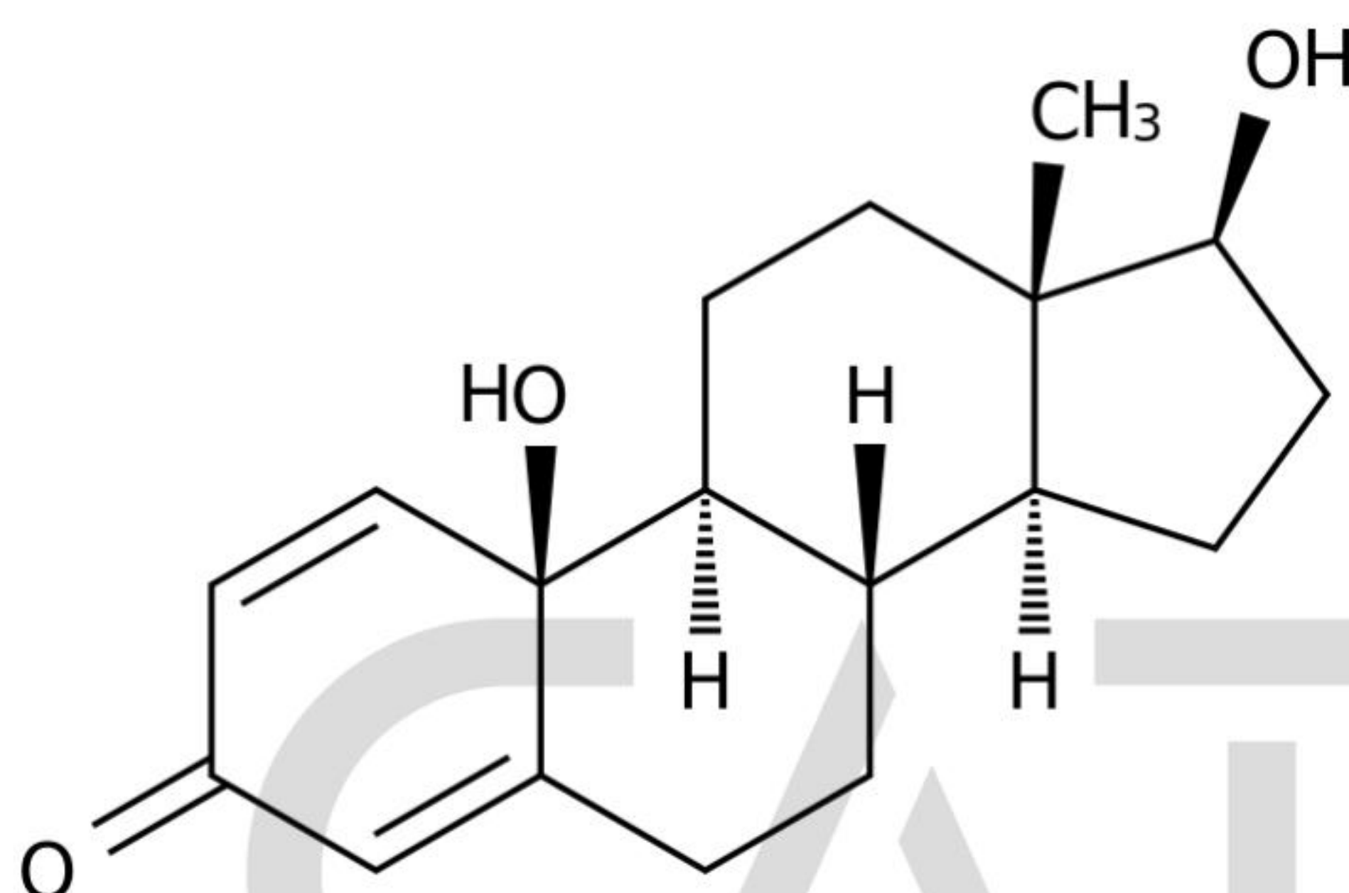
Chemical Structure:
