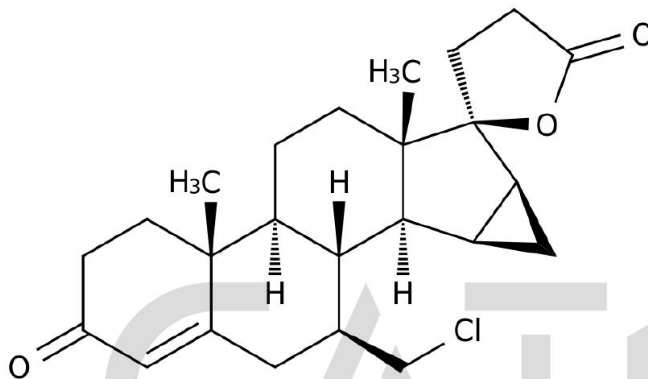
Chemical Structure:
