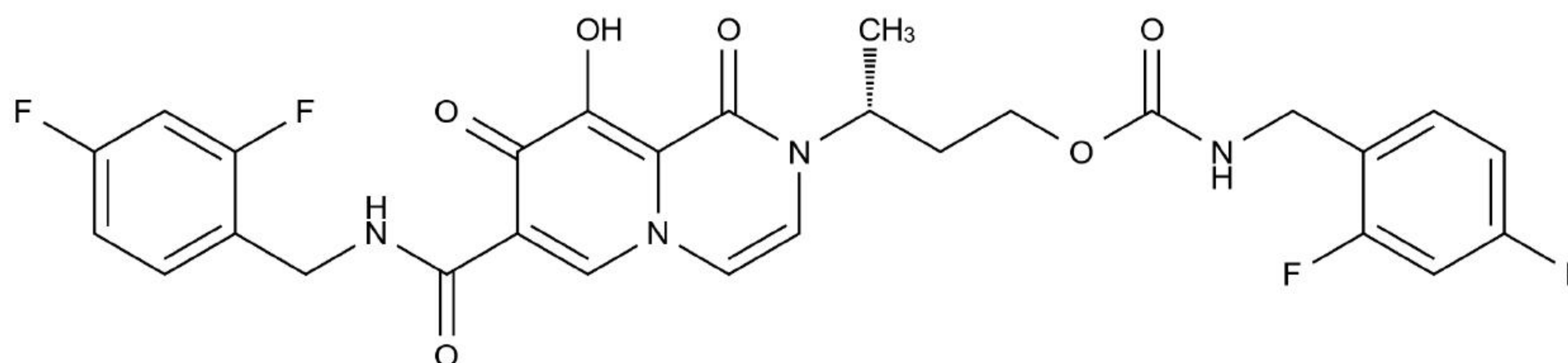
Chemical Structure:
