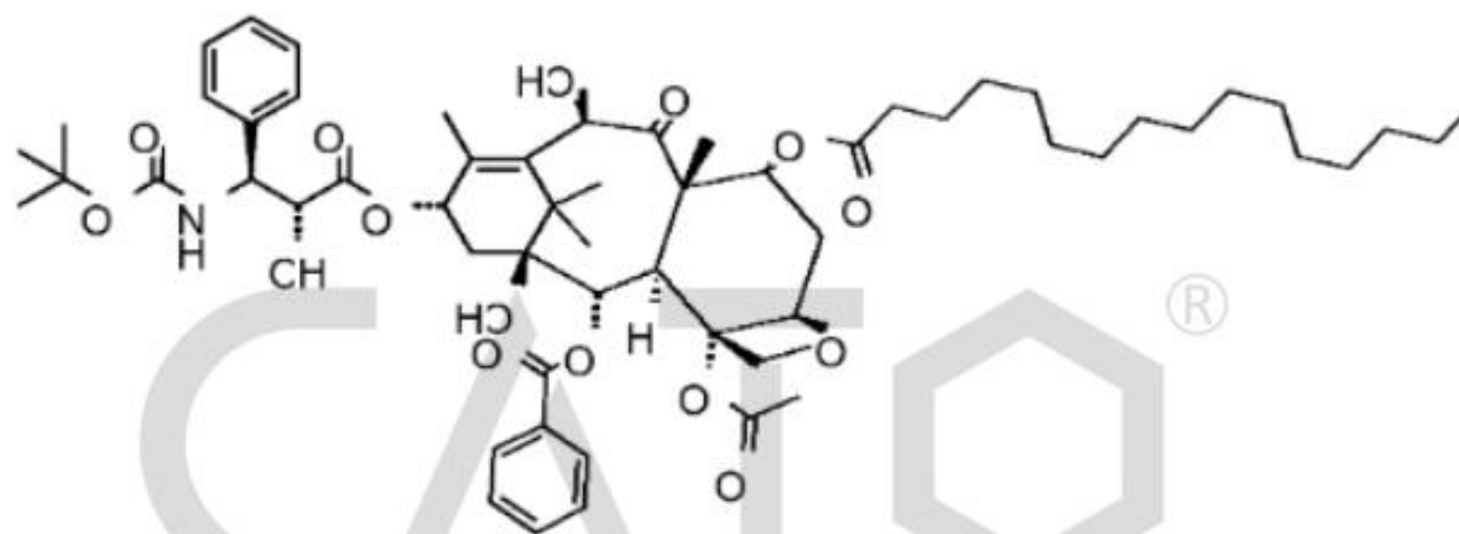
Chemical Structure:
