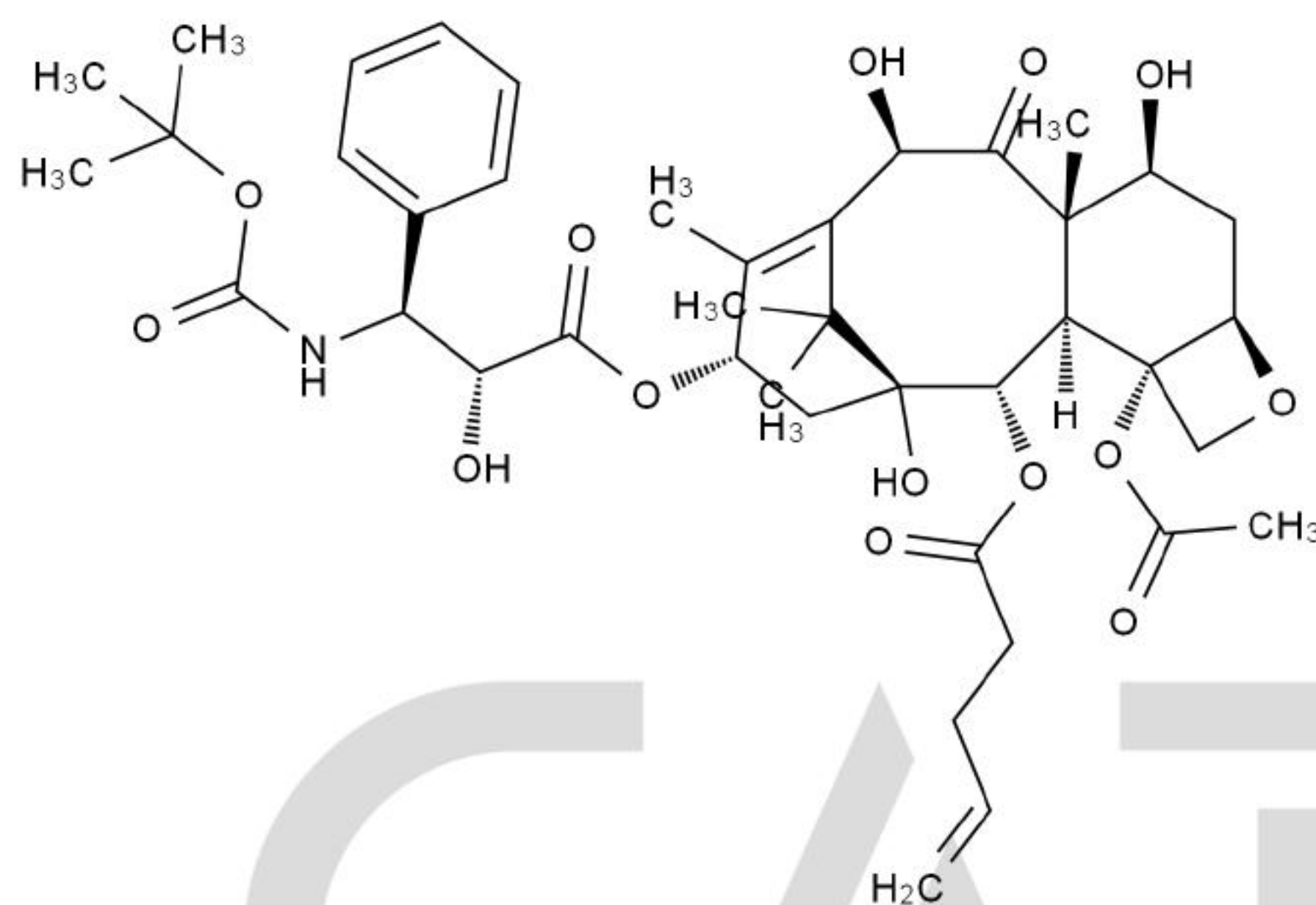
Chemical Structure:
