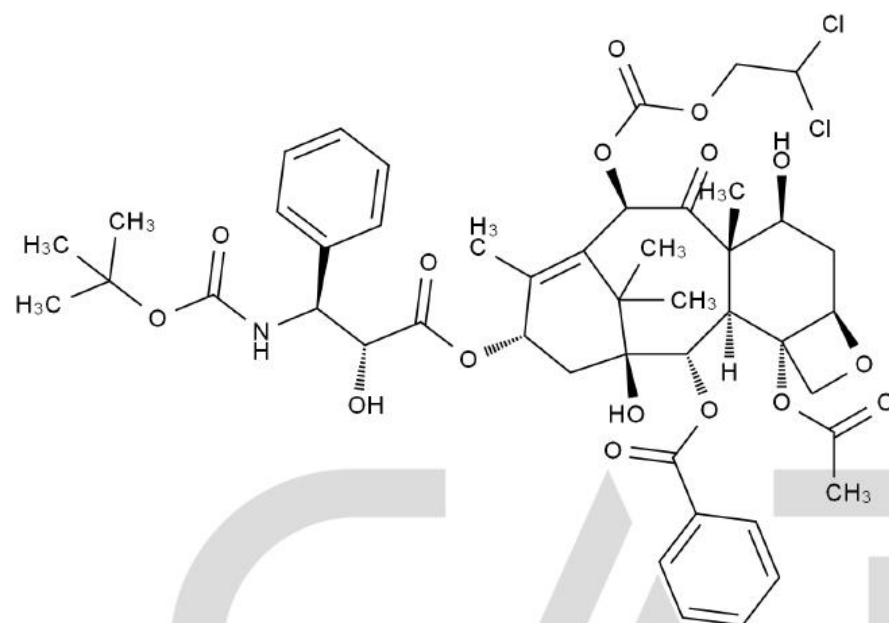
Chemical Structure:
