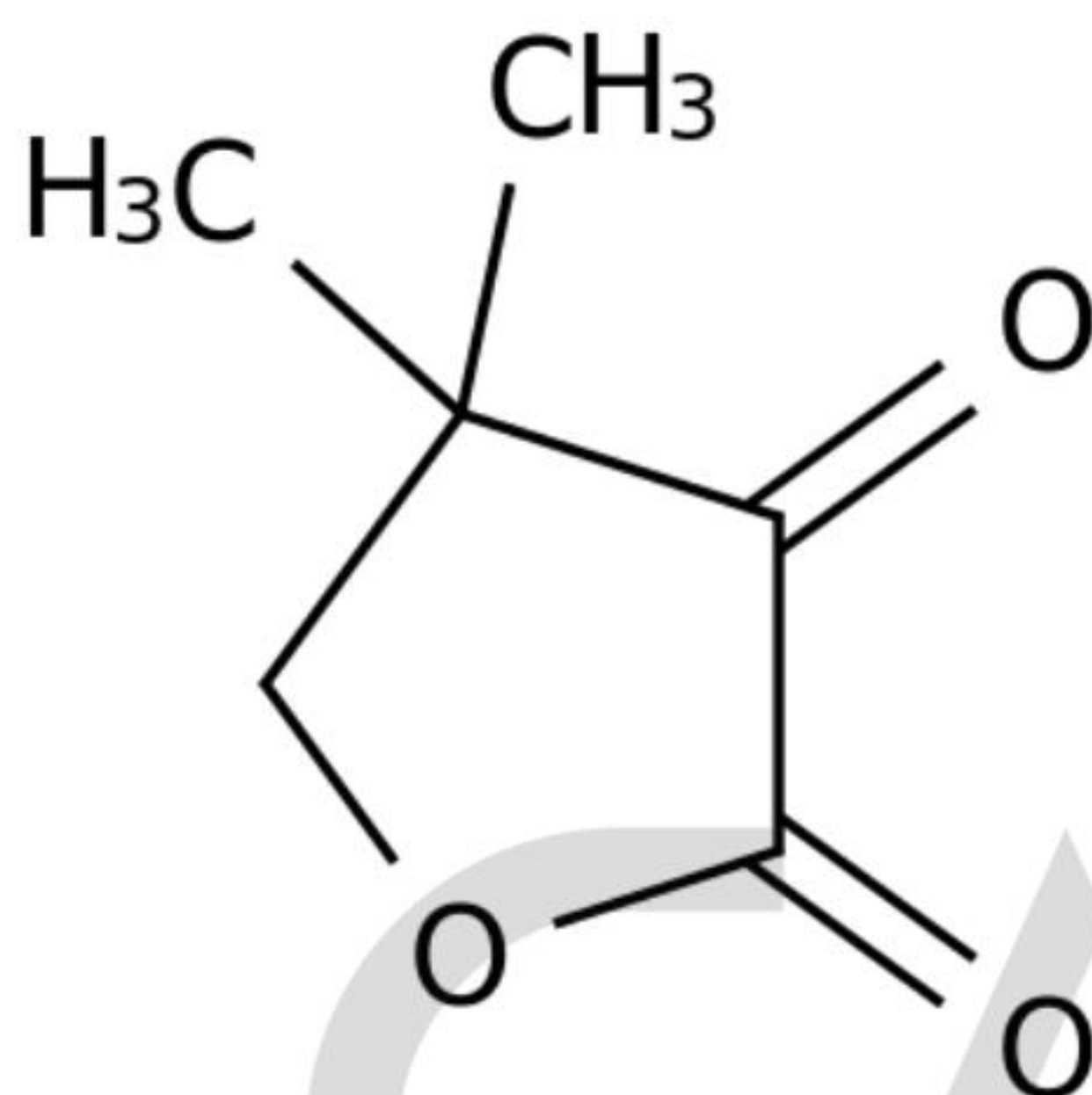
Chemical Structure:
