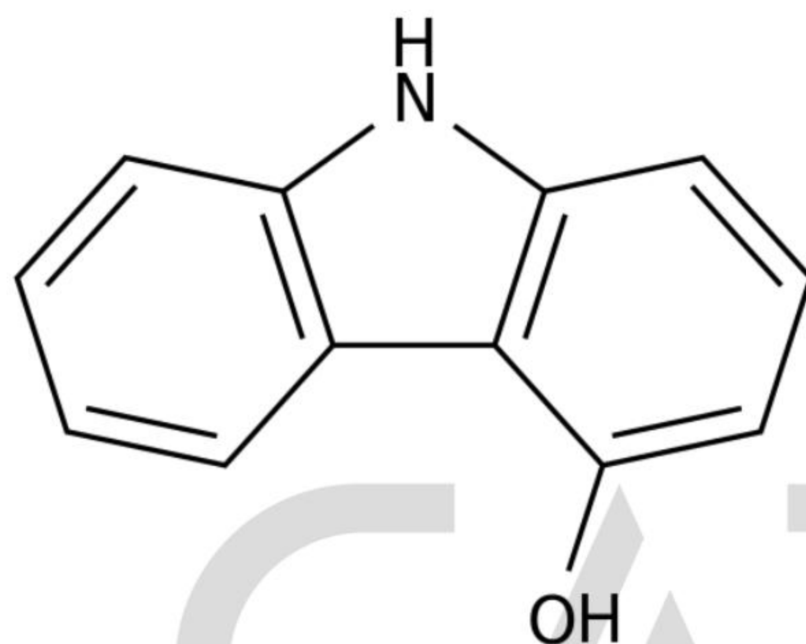
Chemical Structure:
