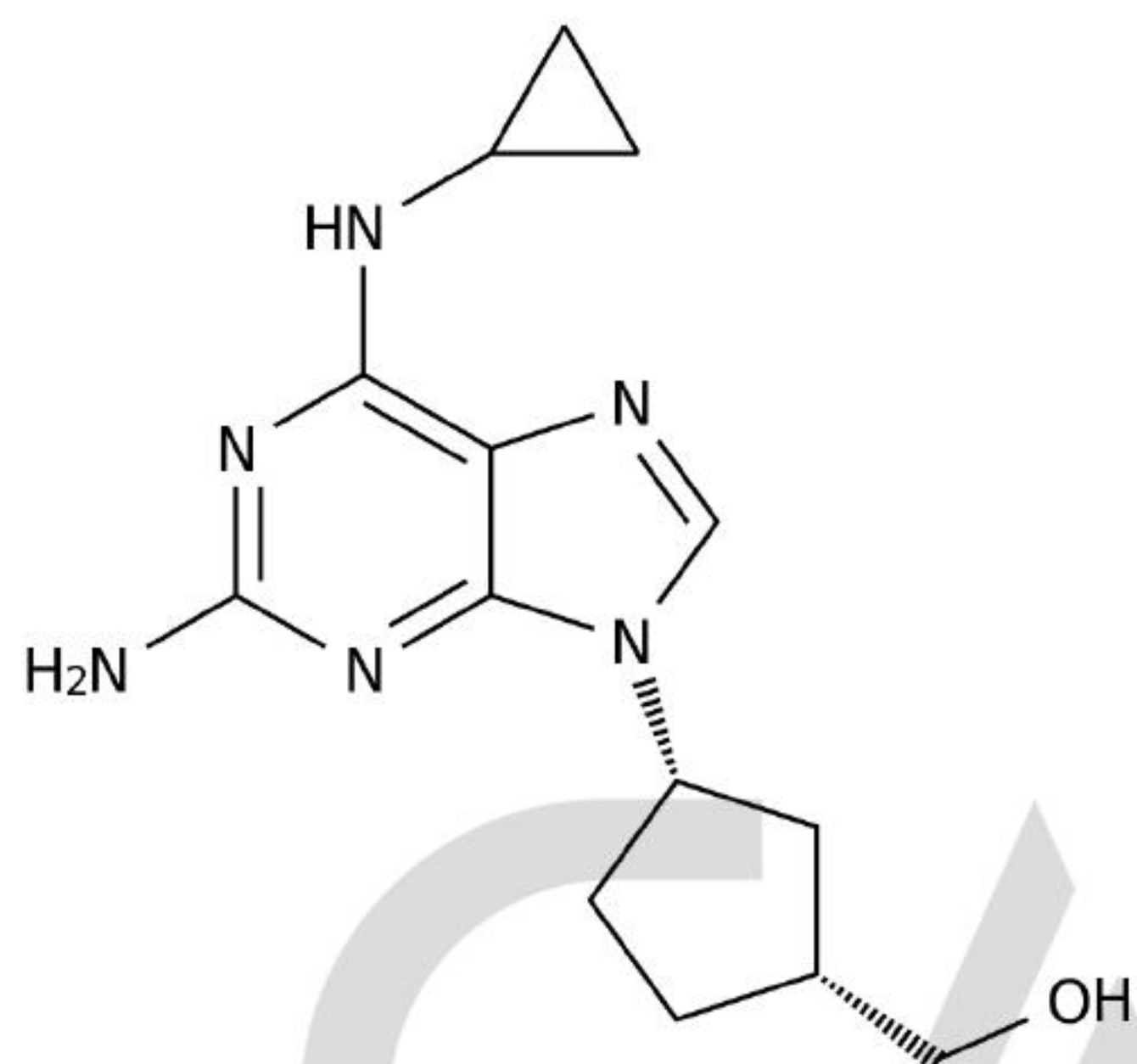
Chemical Structure:
