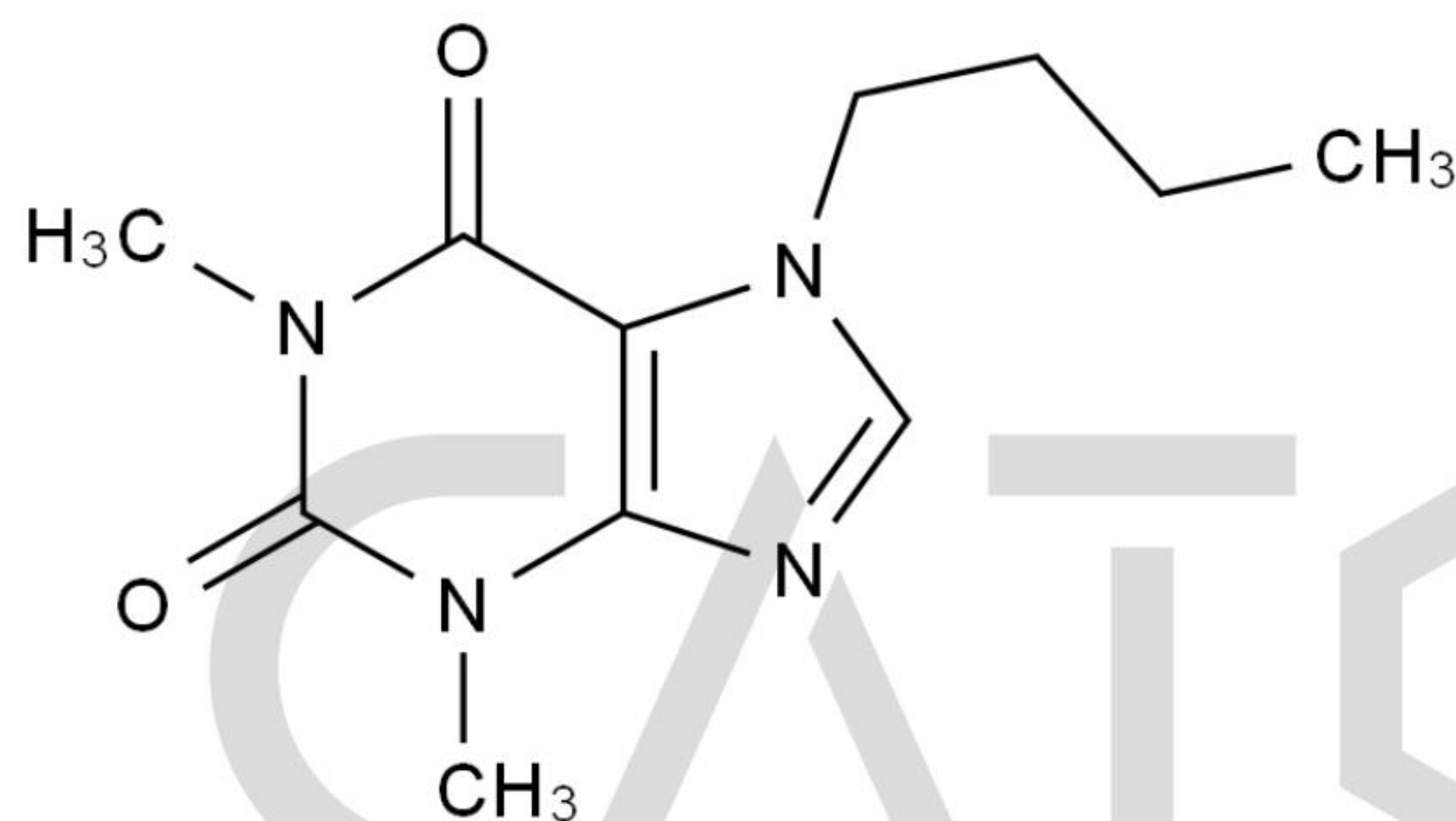
Chemical Structure:
