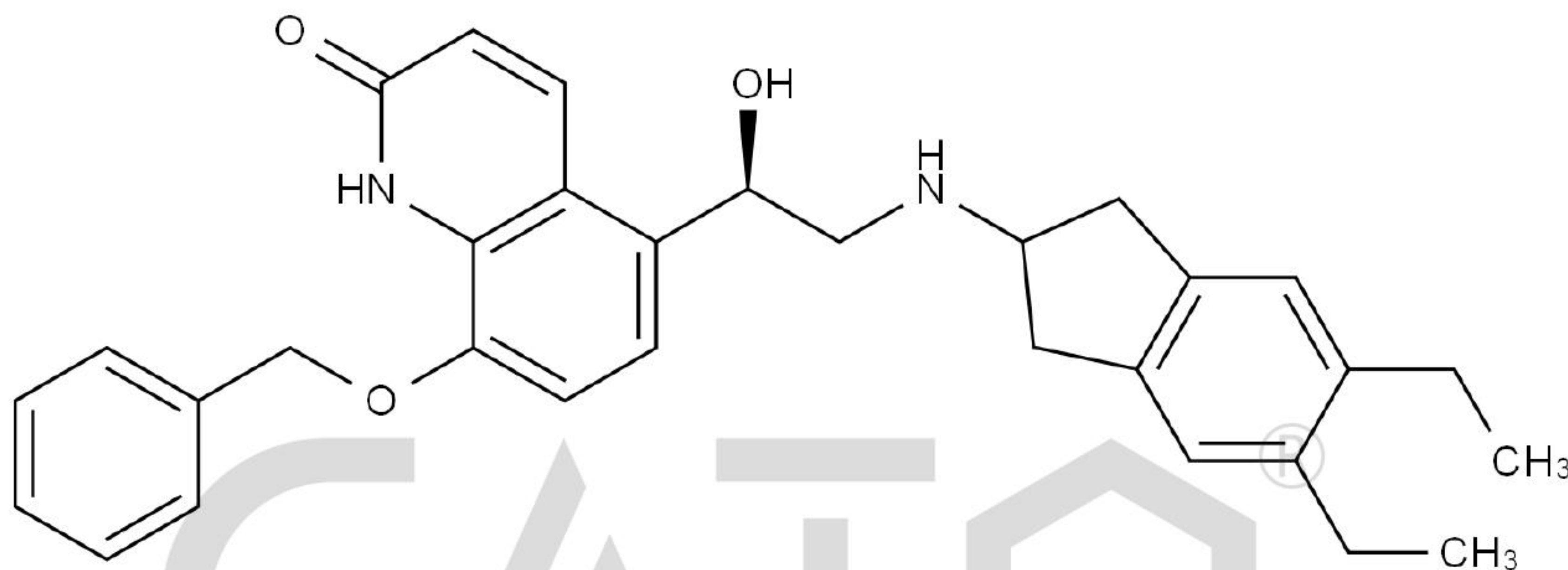
Chemical Structure:
