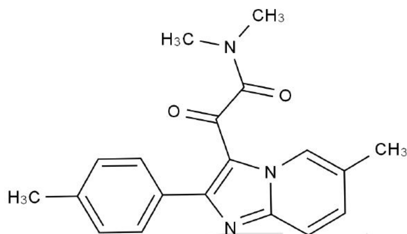
Chemical Structure:
