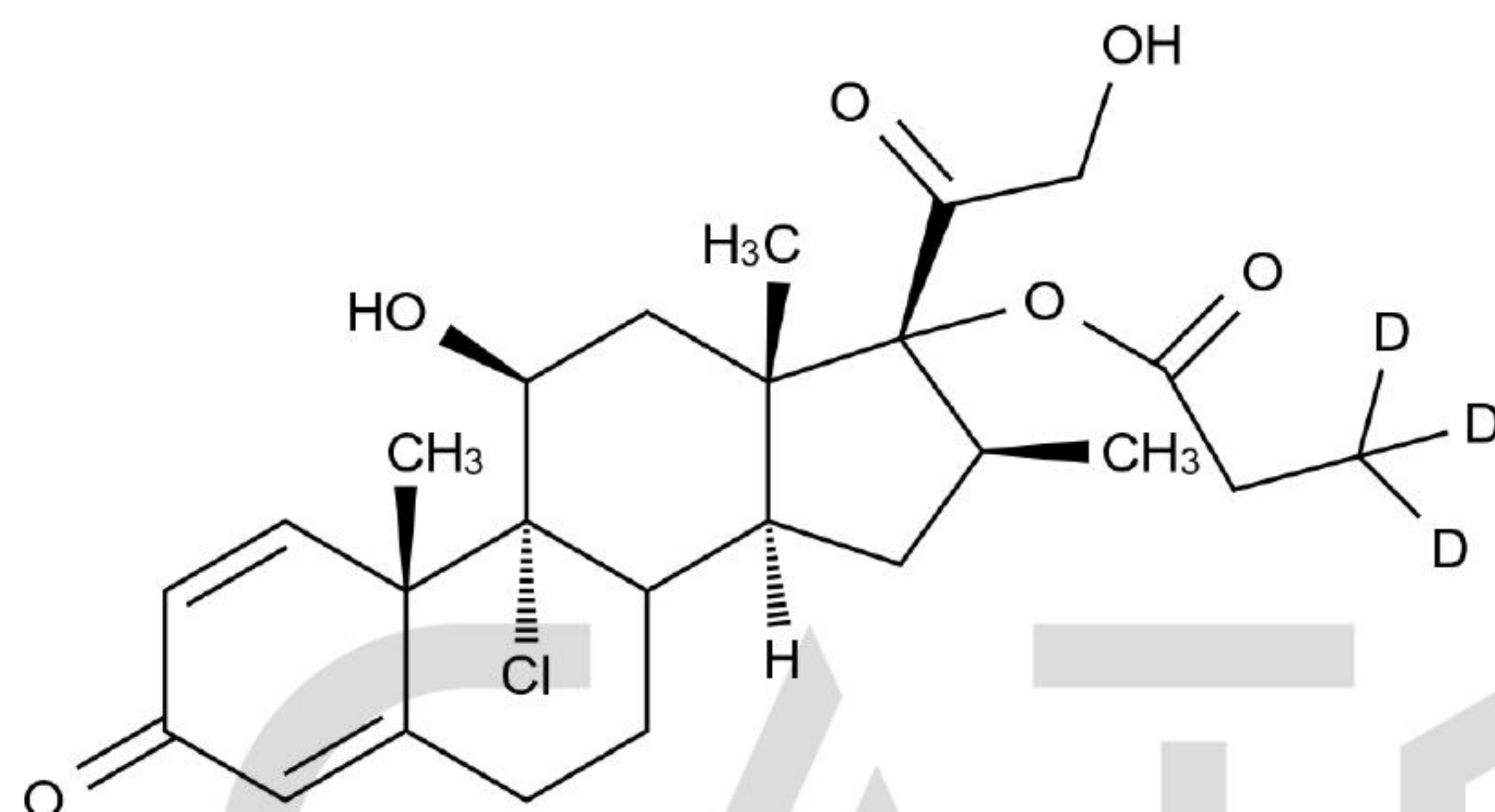
Chemical Structure:
