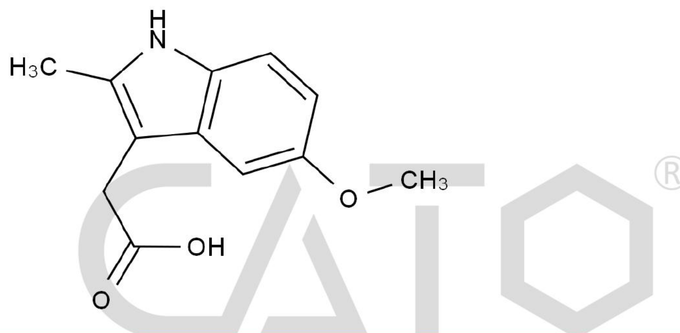
Chemical Structure:
