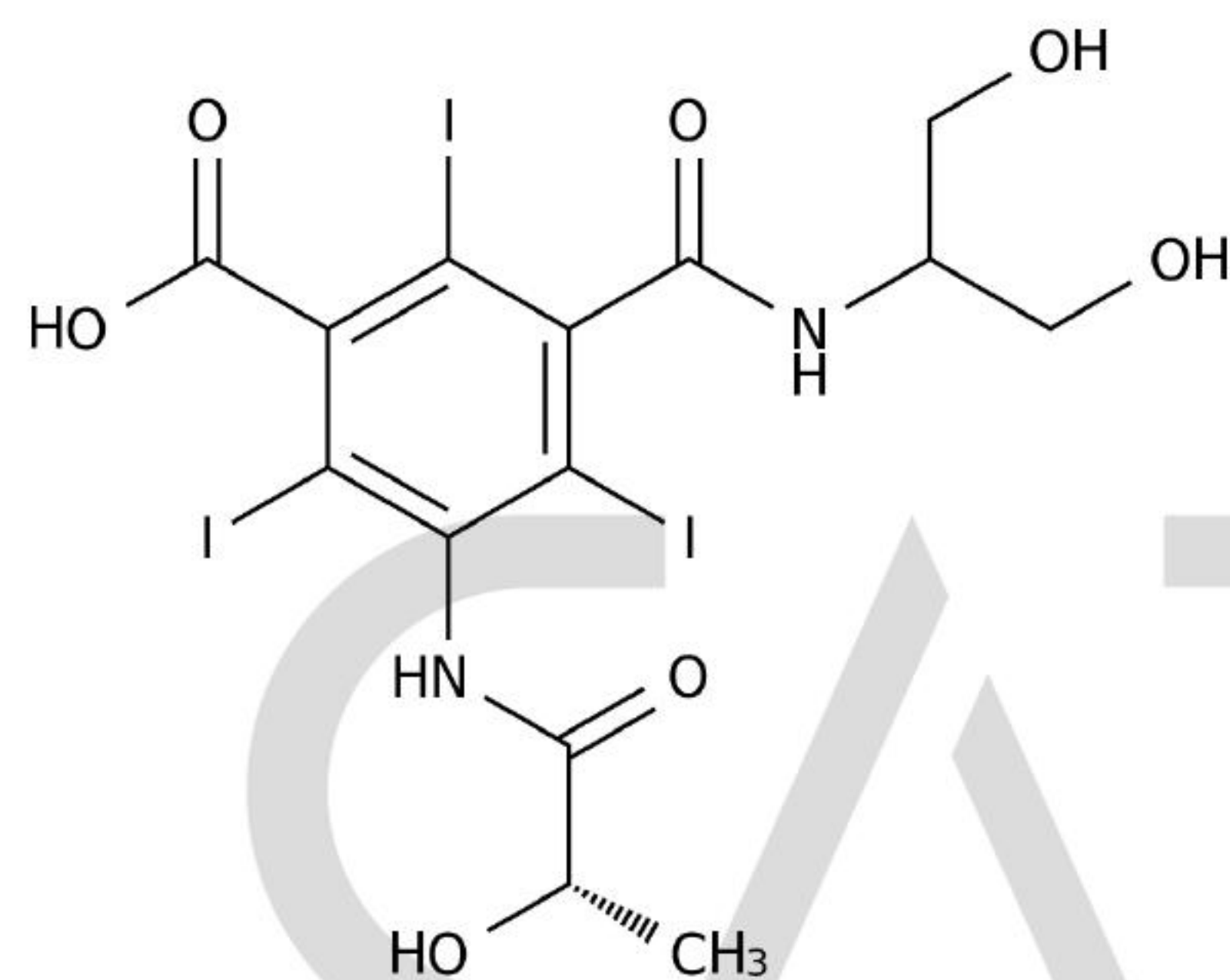
Chemical Structure:
