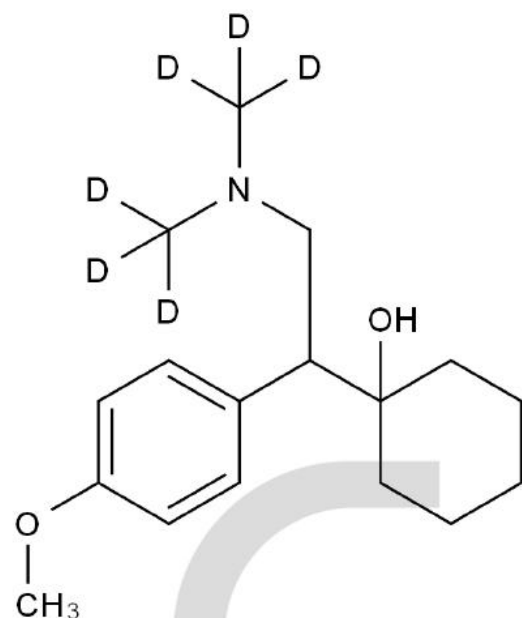
Chemical Structure:
