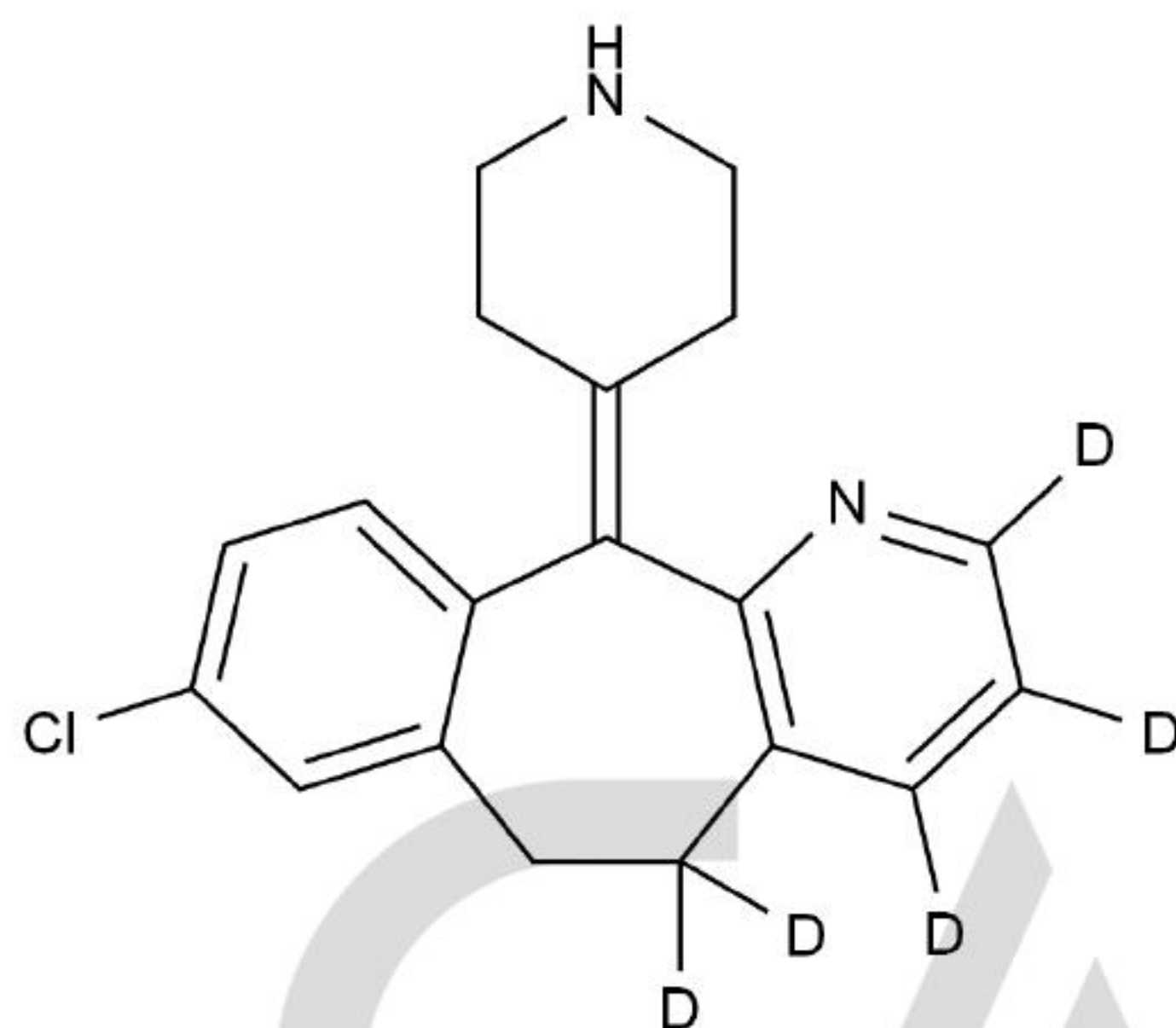
Chemical Structure:
