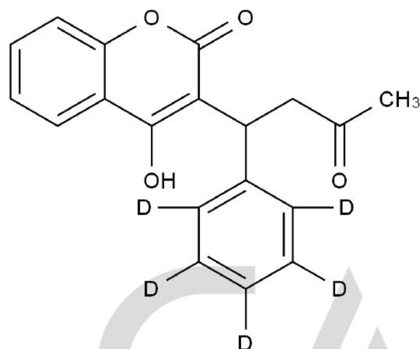
Chemical Structure:
