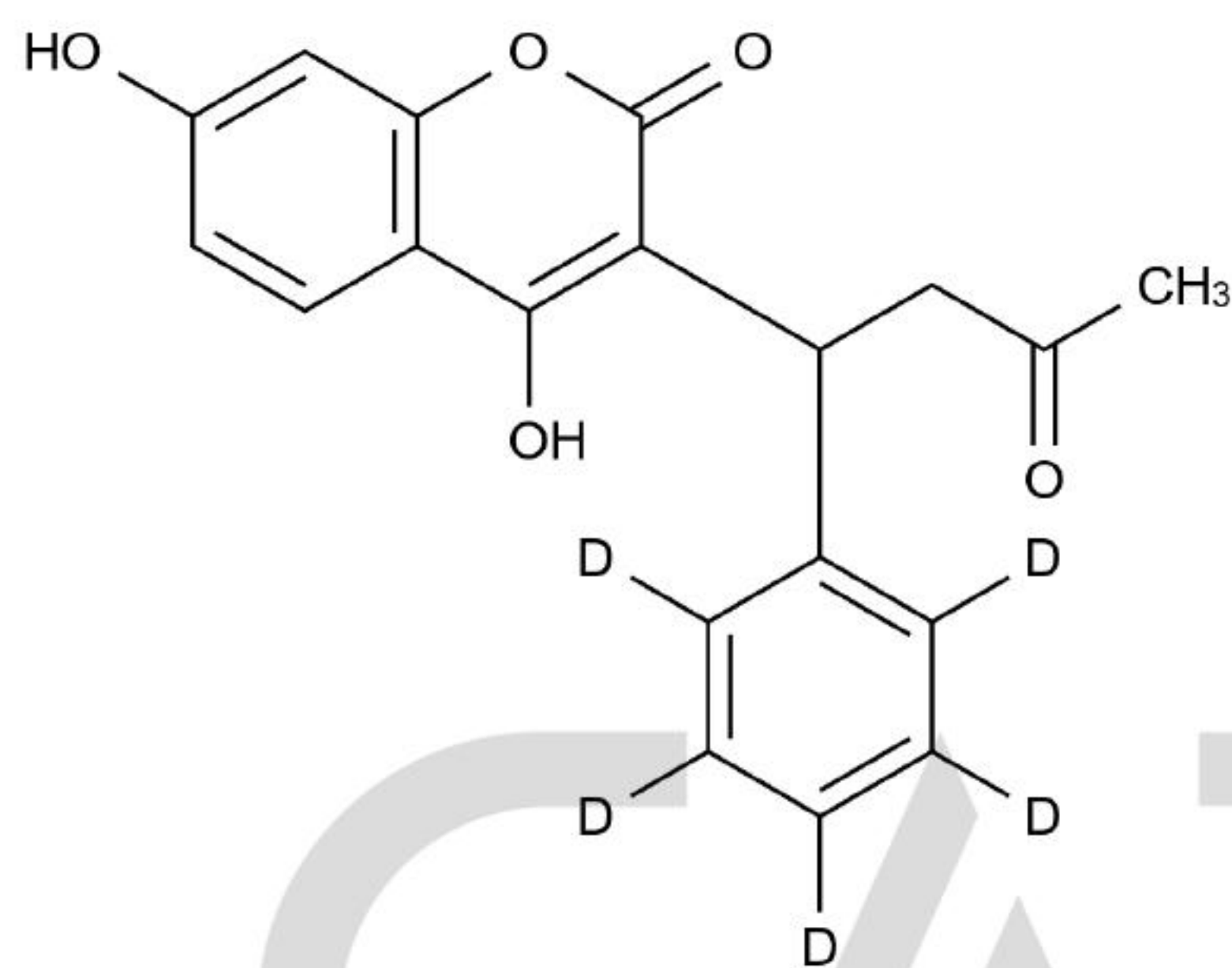
Chemical Structure:
