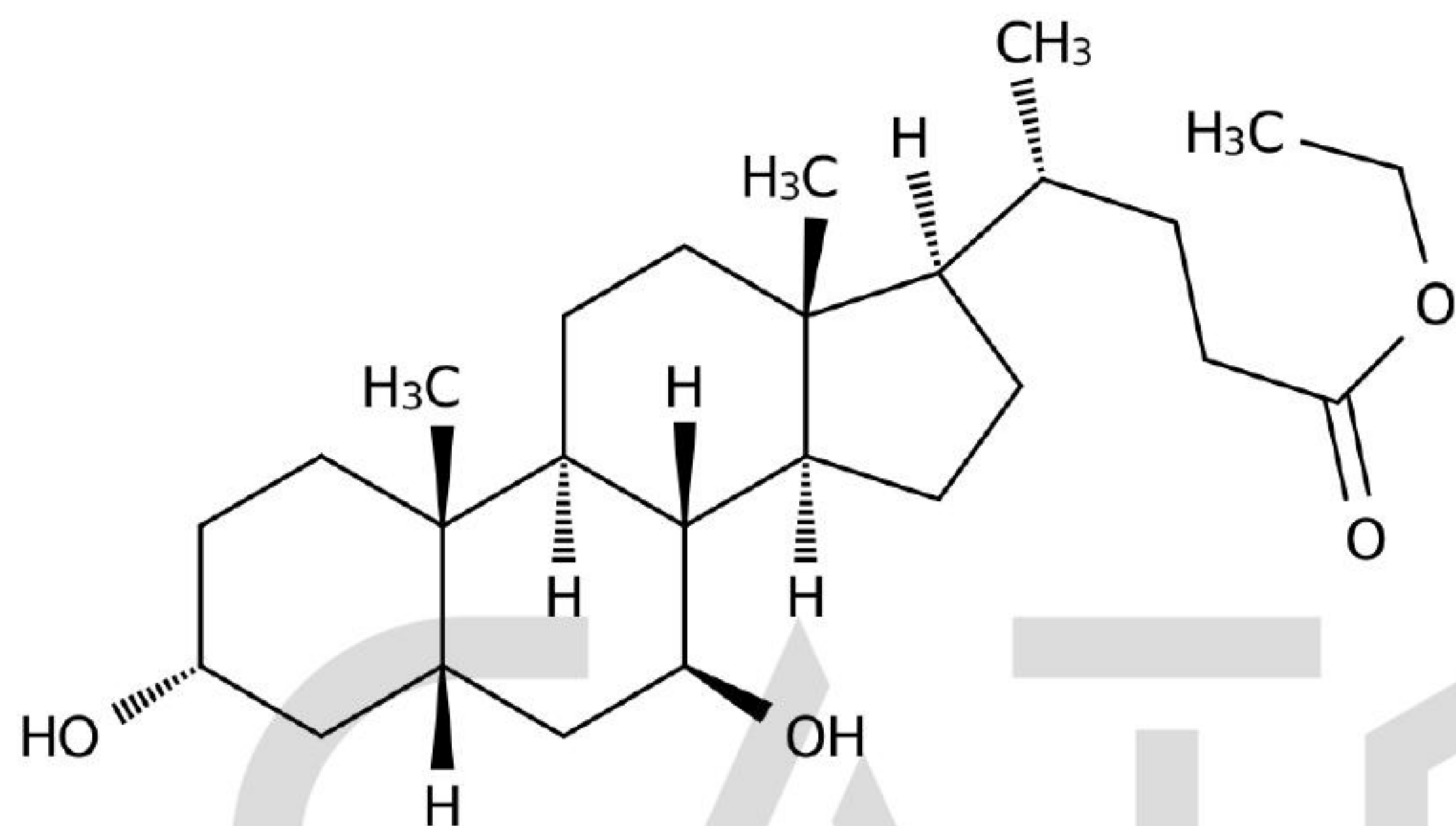
Chemical Structure:
