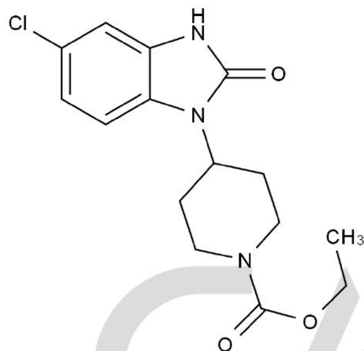
Chemical Structure:
