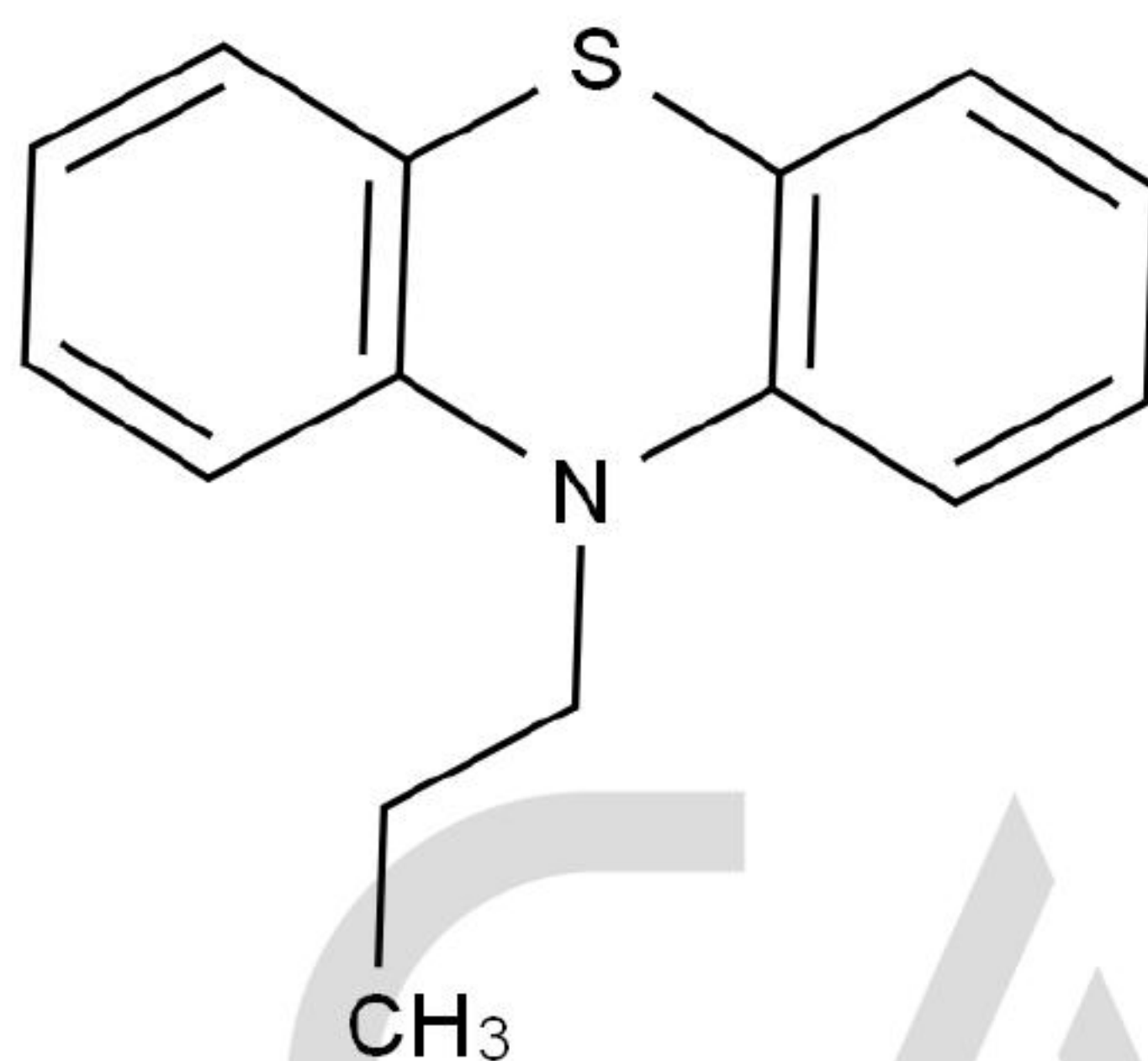
Chemical Structure:
