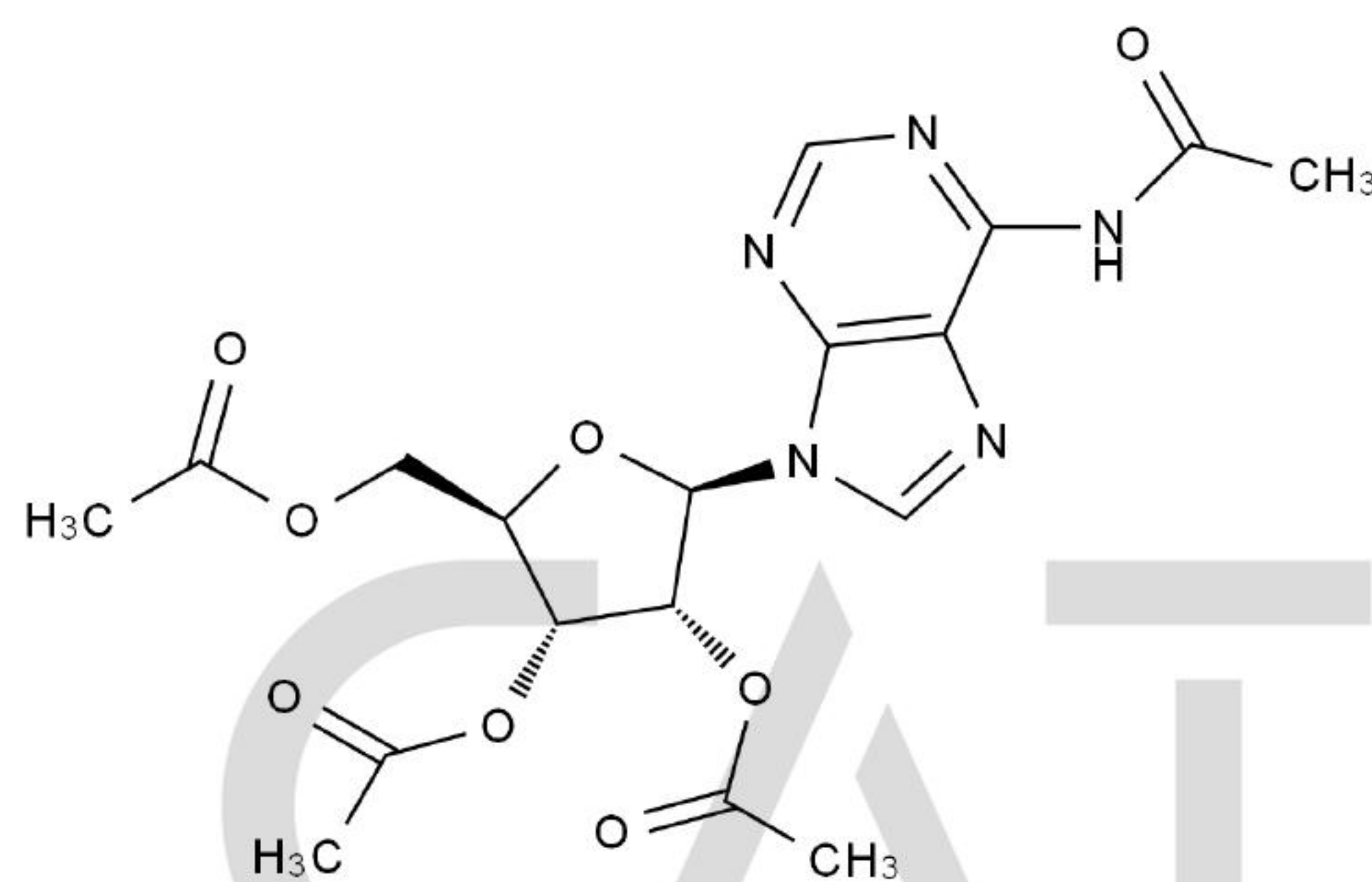
Chemical Structure:
