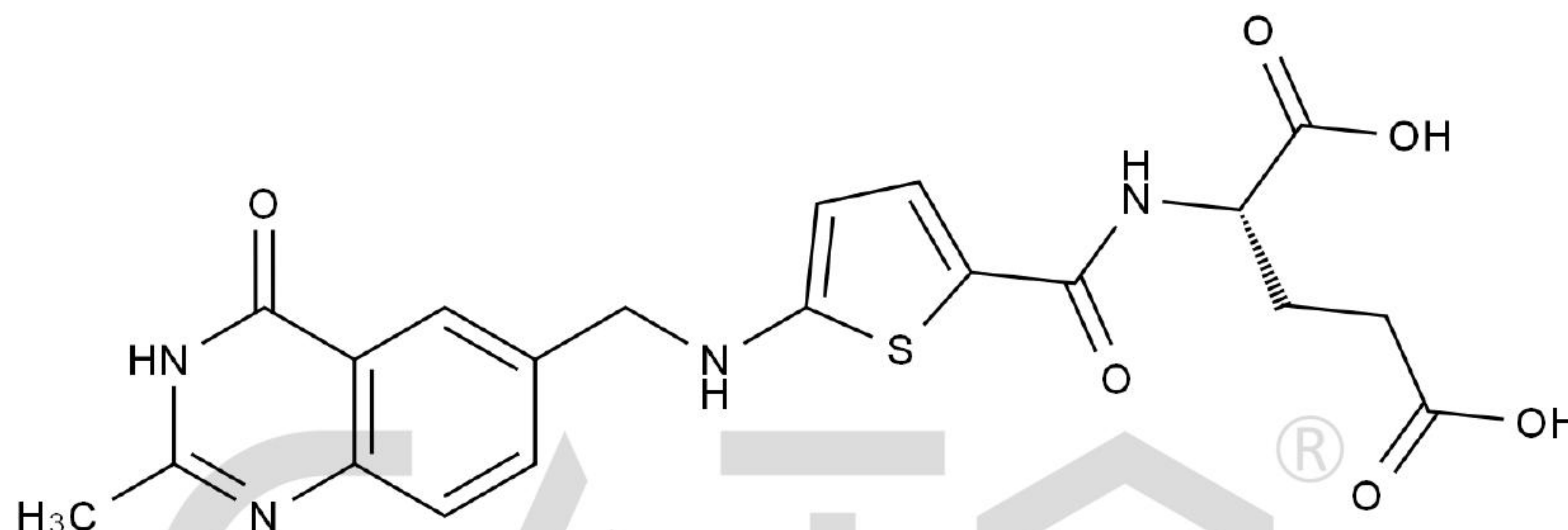
Chemical Structure:
