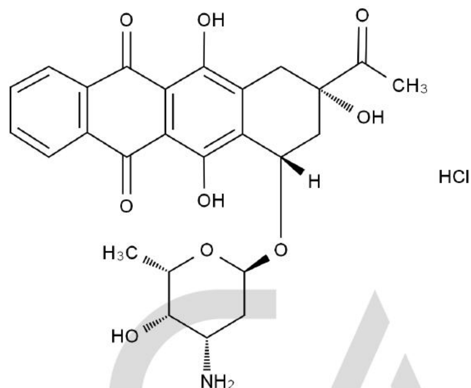
Chemical Structure:
