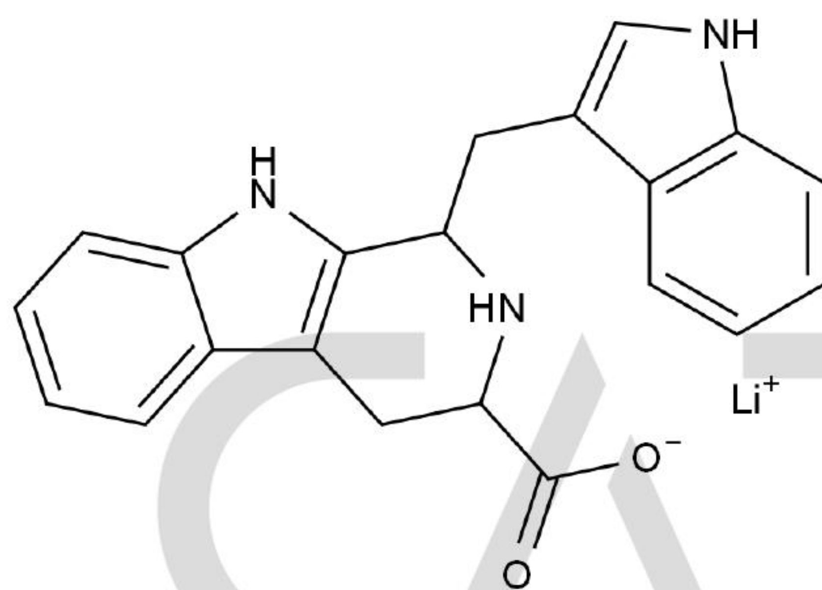
Chemical Structure:
