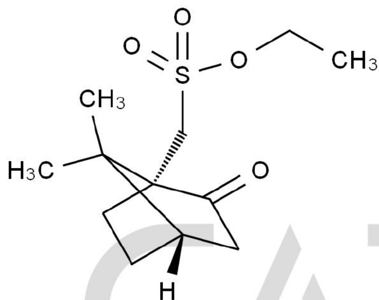
Chemical Structure:
