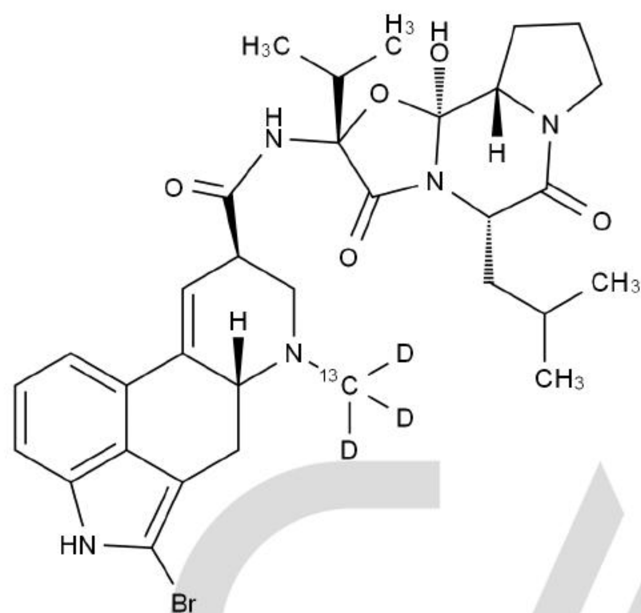
Chemical Structure:
