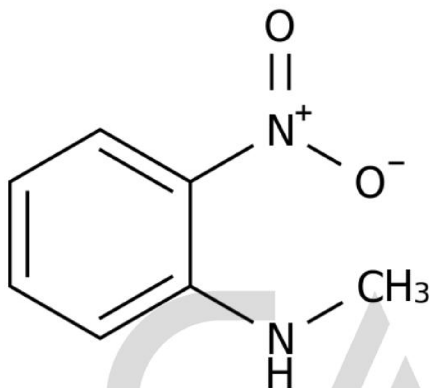
Chemical Structure:
