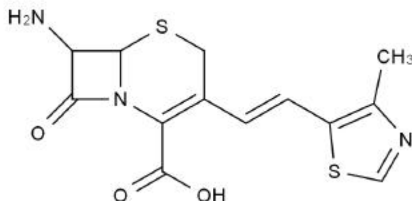
Chemical Structure:
