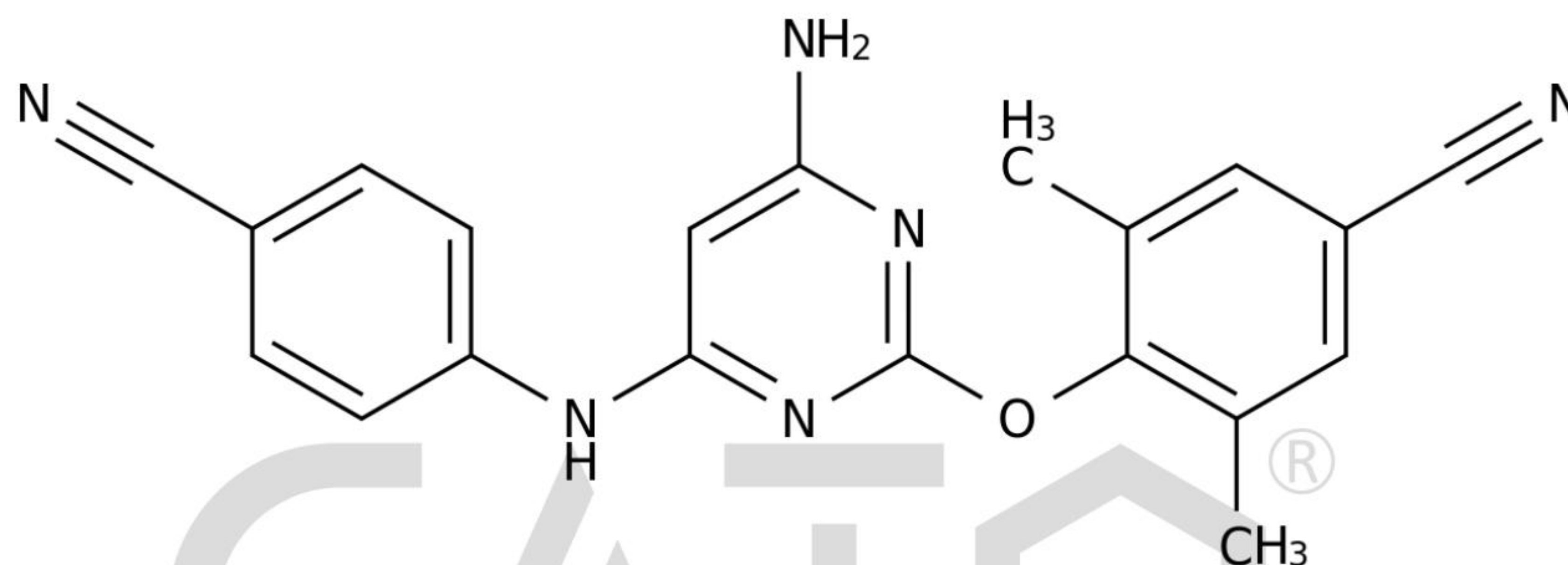
Chemical Structure:
