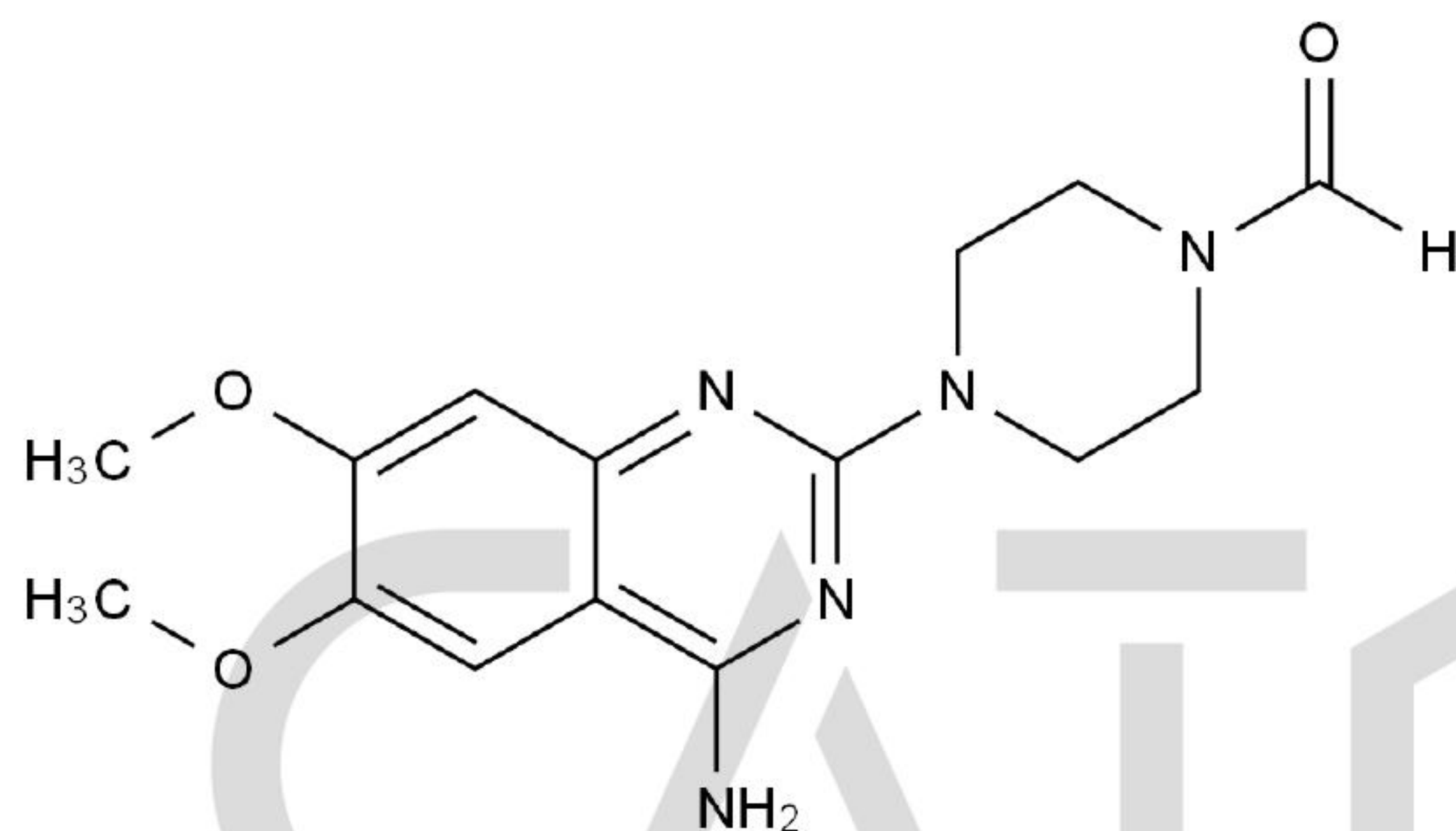
Chemical Structure:
