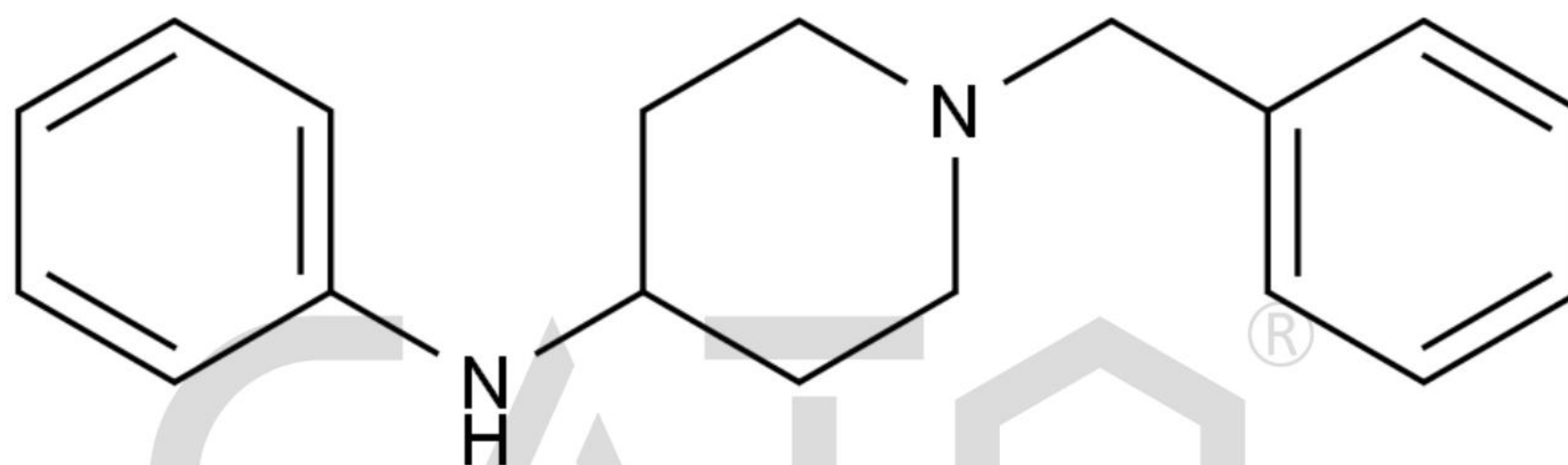
Chemical Structure:
