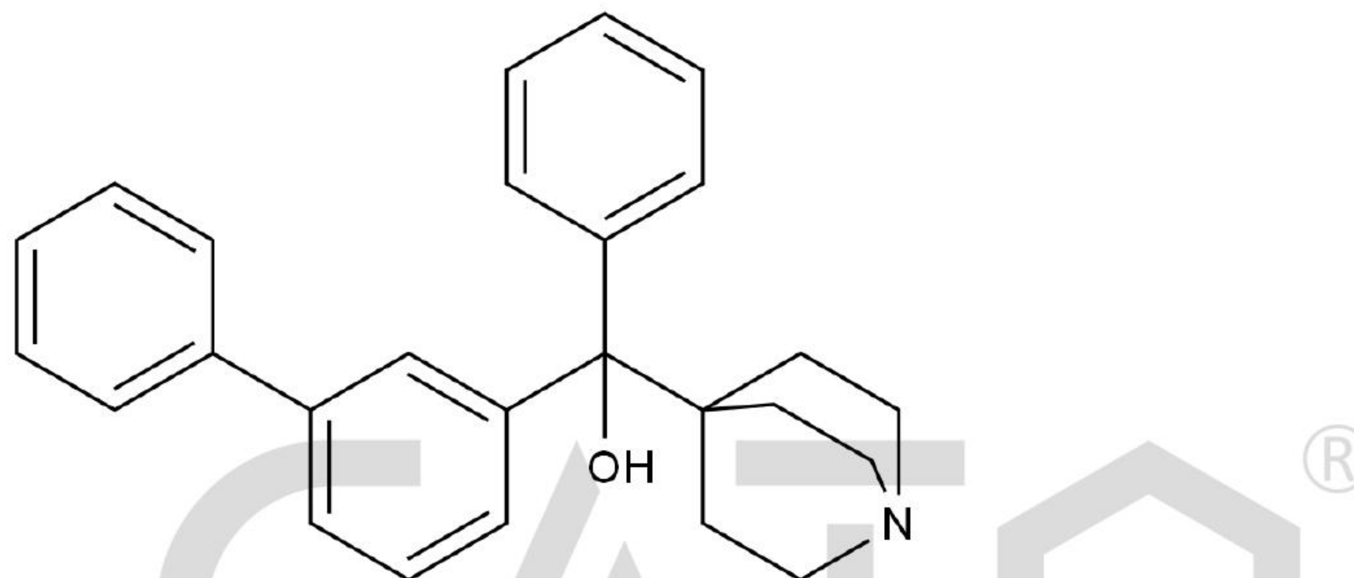
Chemical Structure:
