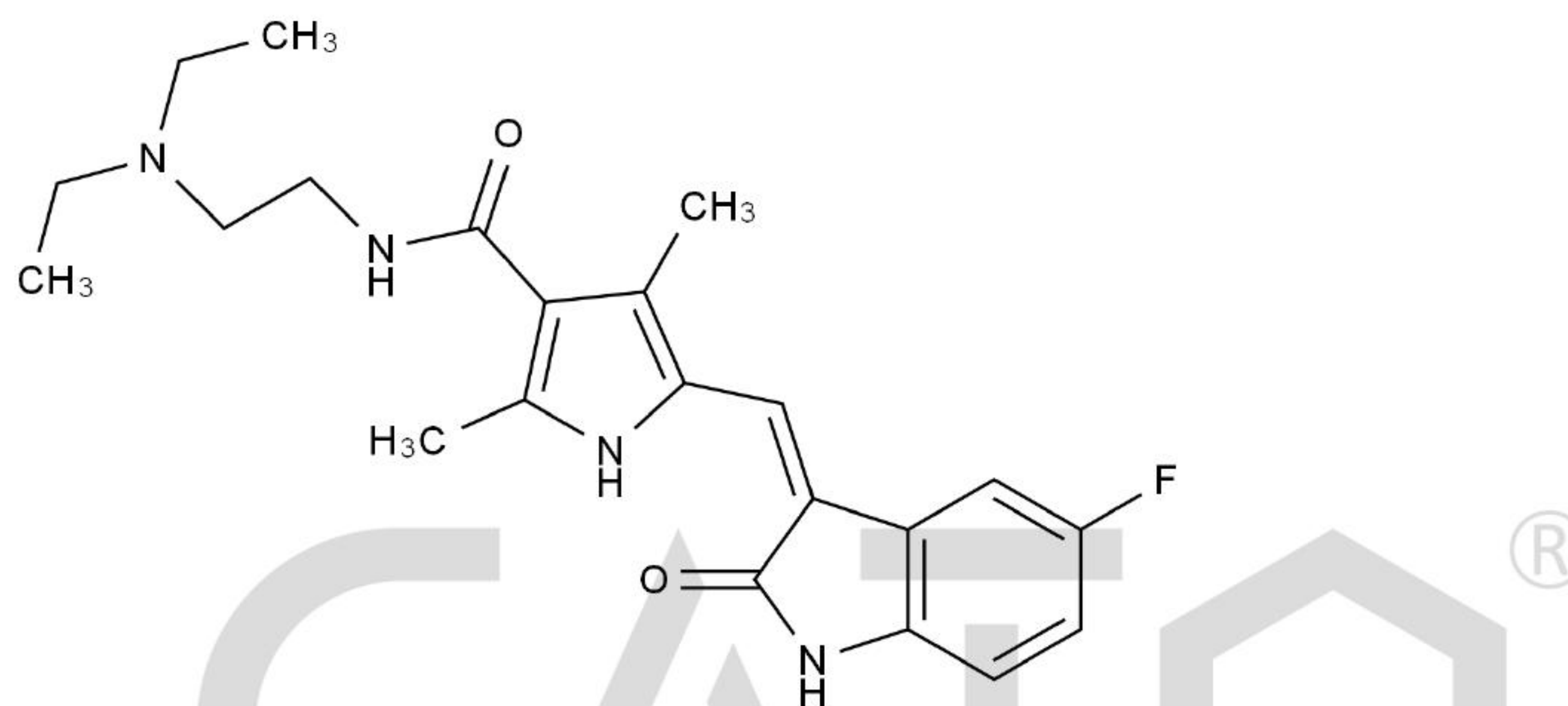
Chemical Structure:
