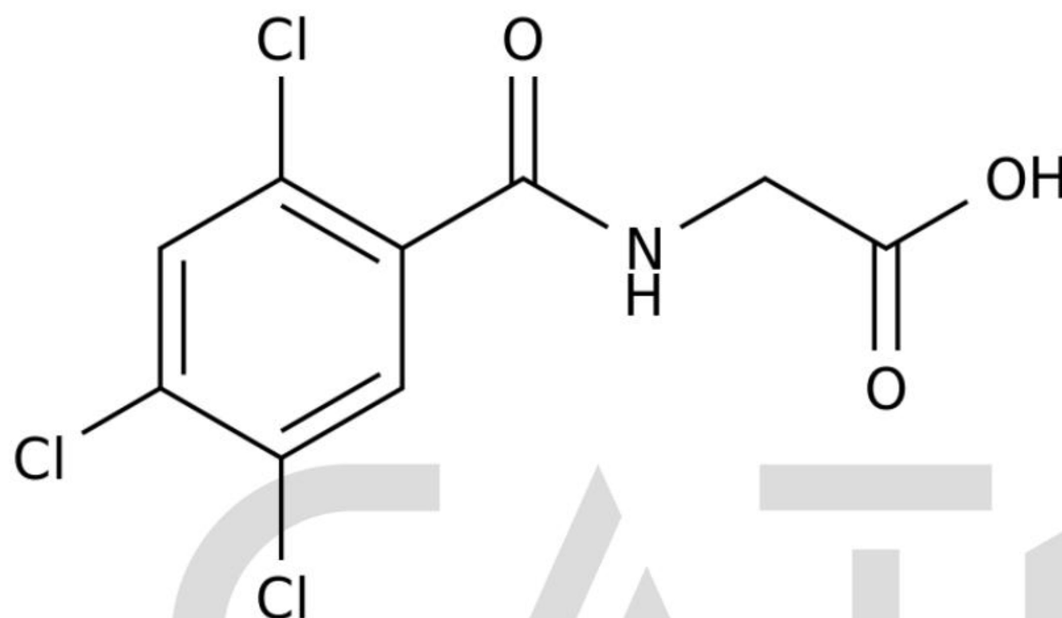
Chemical Structure:
