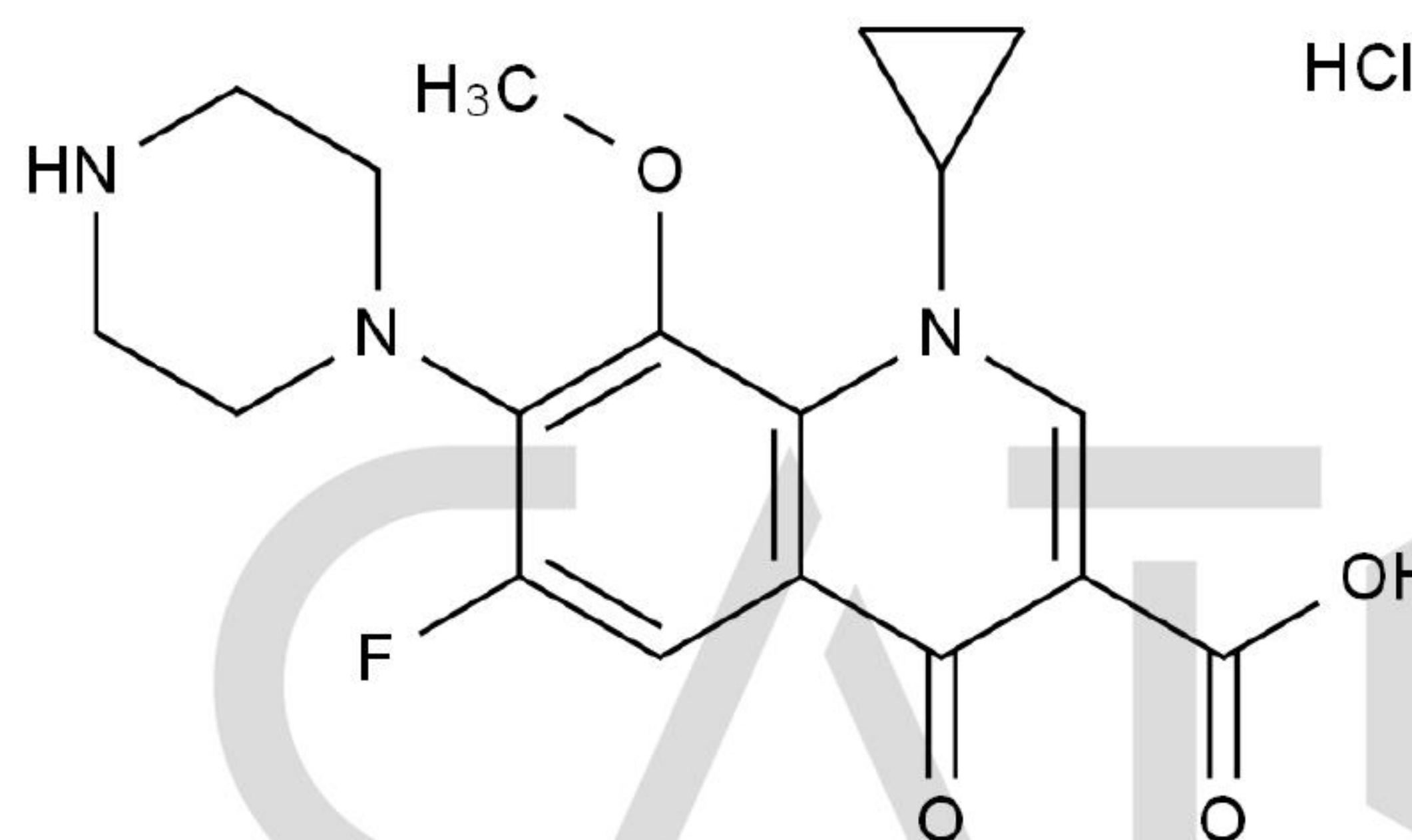
Chemical Structure:
