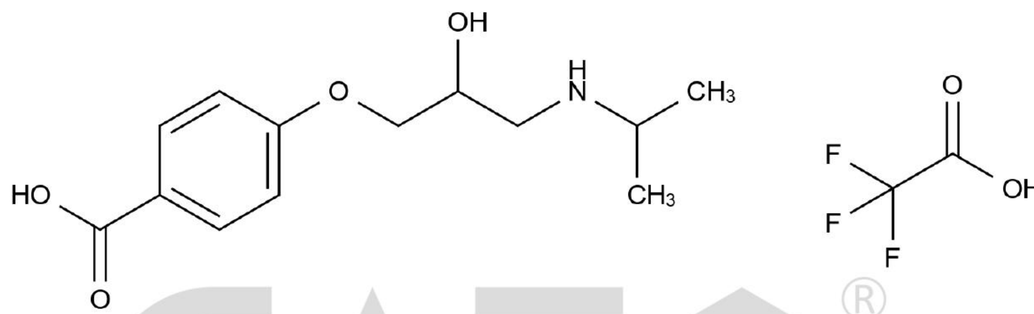
Chemical Structure:
