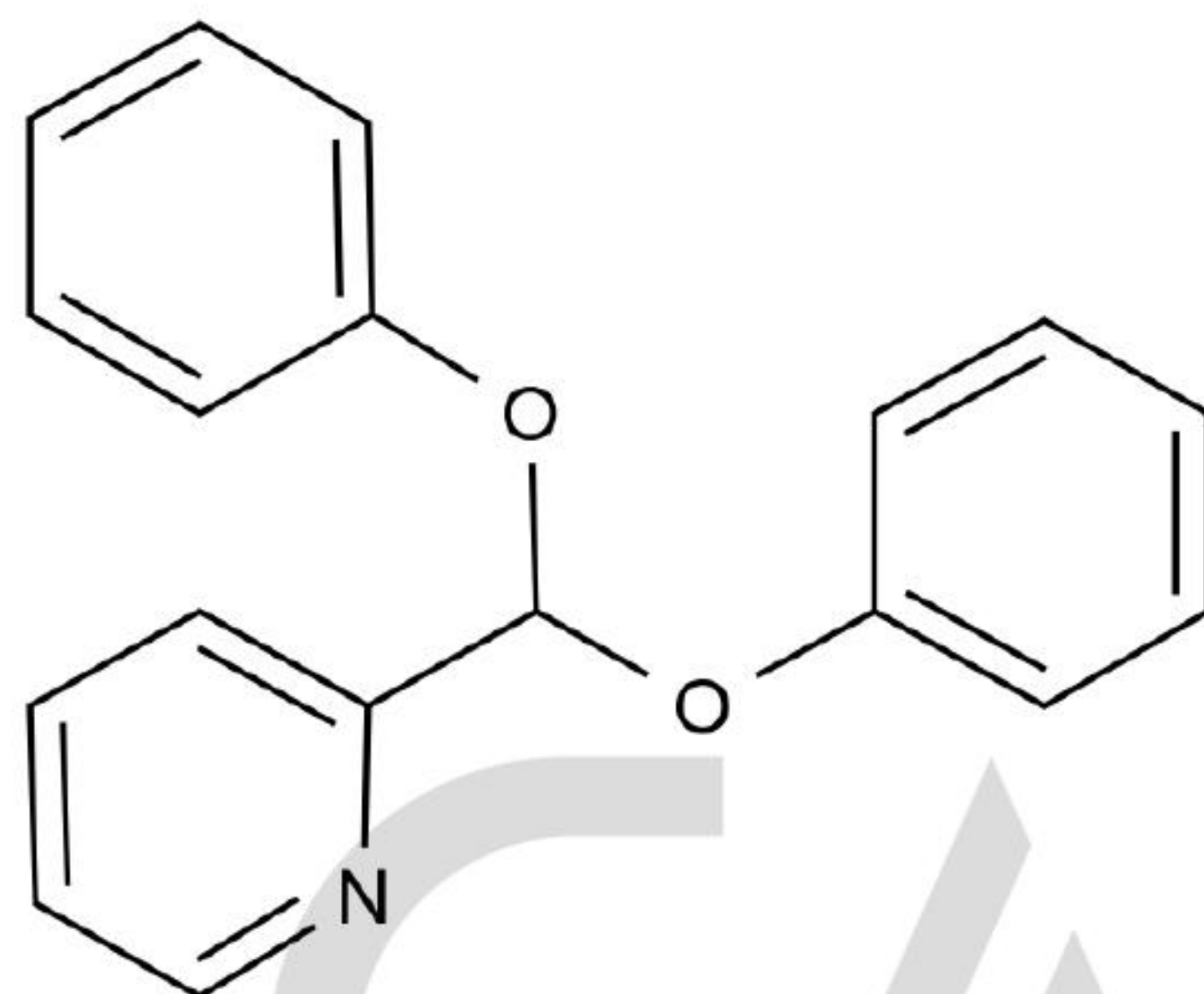
Chemical Structure:
