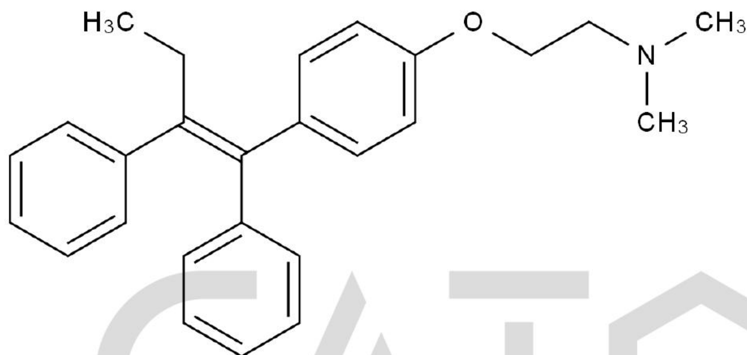
Chemical Structure:
