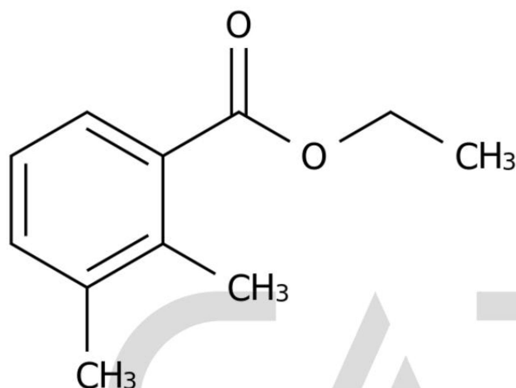
Chemical Structure:
