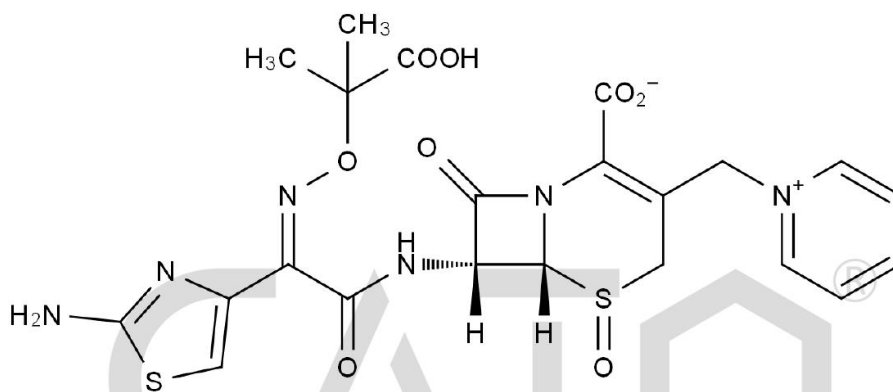
Chemical Structure:
