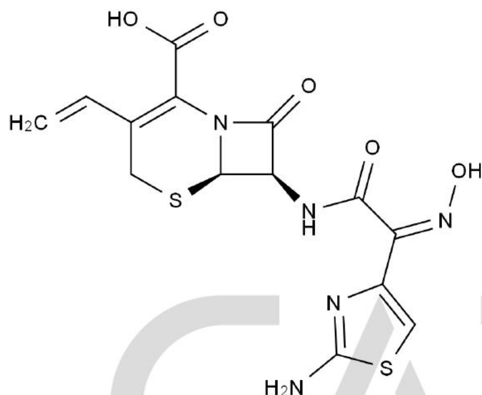
Chemical Structure:
