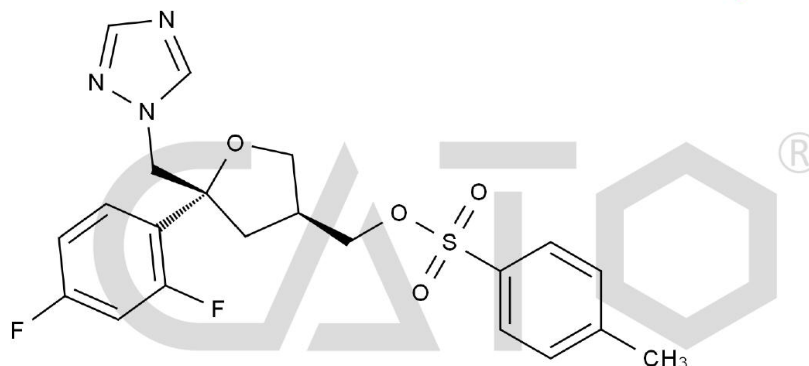
Chemical Structure:
